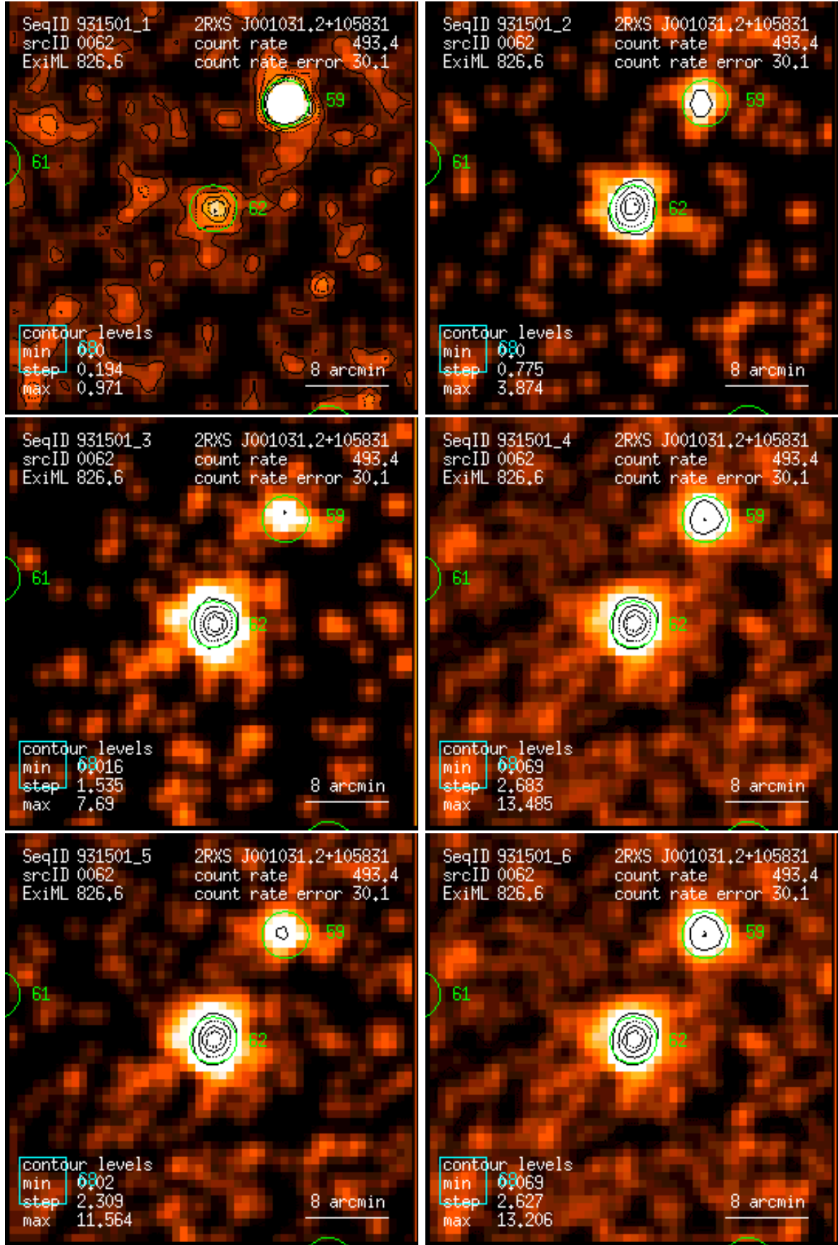
Figure 62: RASS 931501: detection 0062: band rate images, Gaussian filter: (1) PSPC channels 11 – 41, (2) 52 – 90, (3) 91 – 201, (4) 11 – 235, (5) 52 – 201, (6) 11 – 201. Broad band rates in counts/ks. Band rate contour levels in counts/ks/arcmin 2 .
