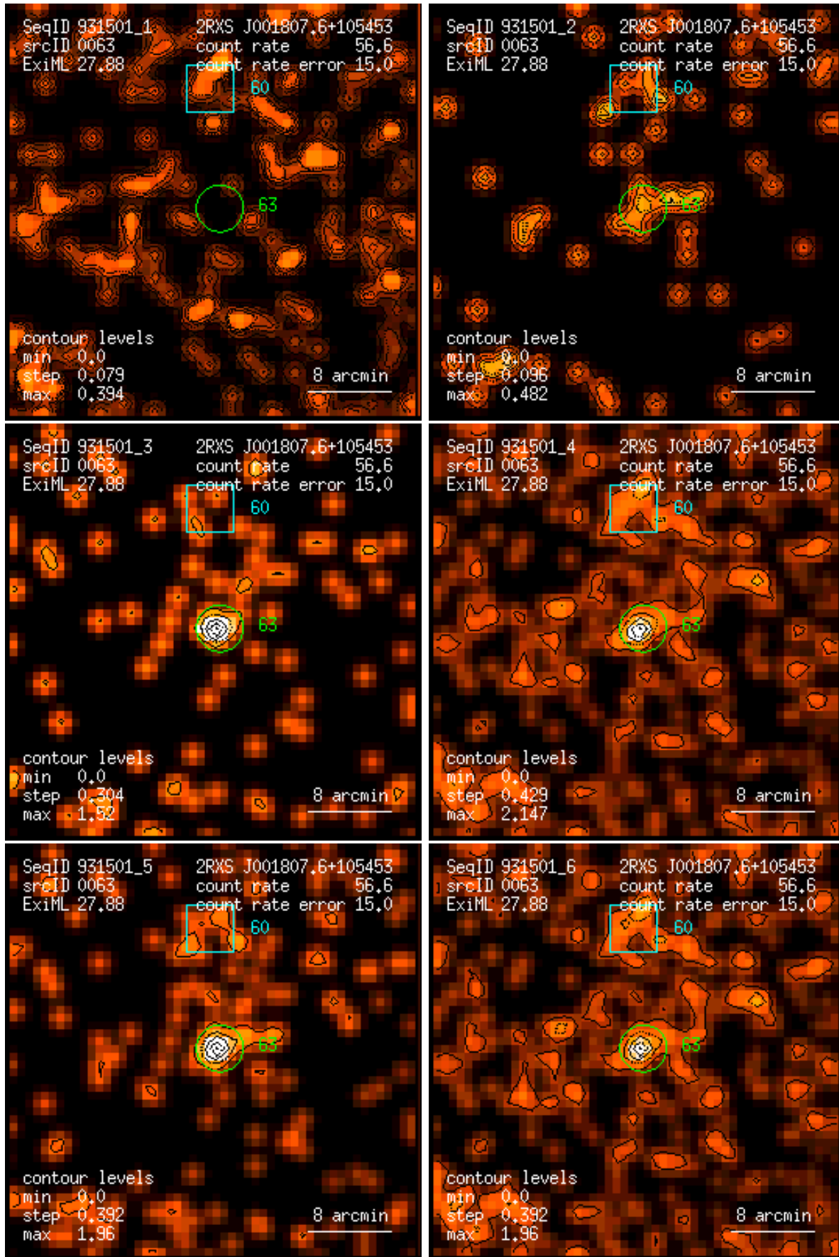
Figure 63: RASS 931501: detection 0063: band rate images, Gaussian filter: (1) PSPC channels 11 – 41, (2) 52 – 90, (3) 91 – 201, (4) 11 – 235, (5) 52 – 201, (6) 11 – 201. Broad band rates in counts/ks. Band rate contour levels in counts/ks/arcmin 2 .
