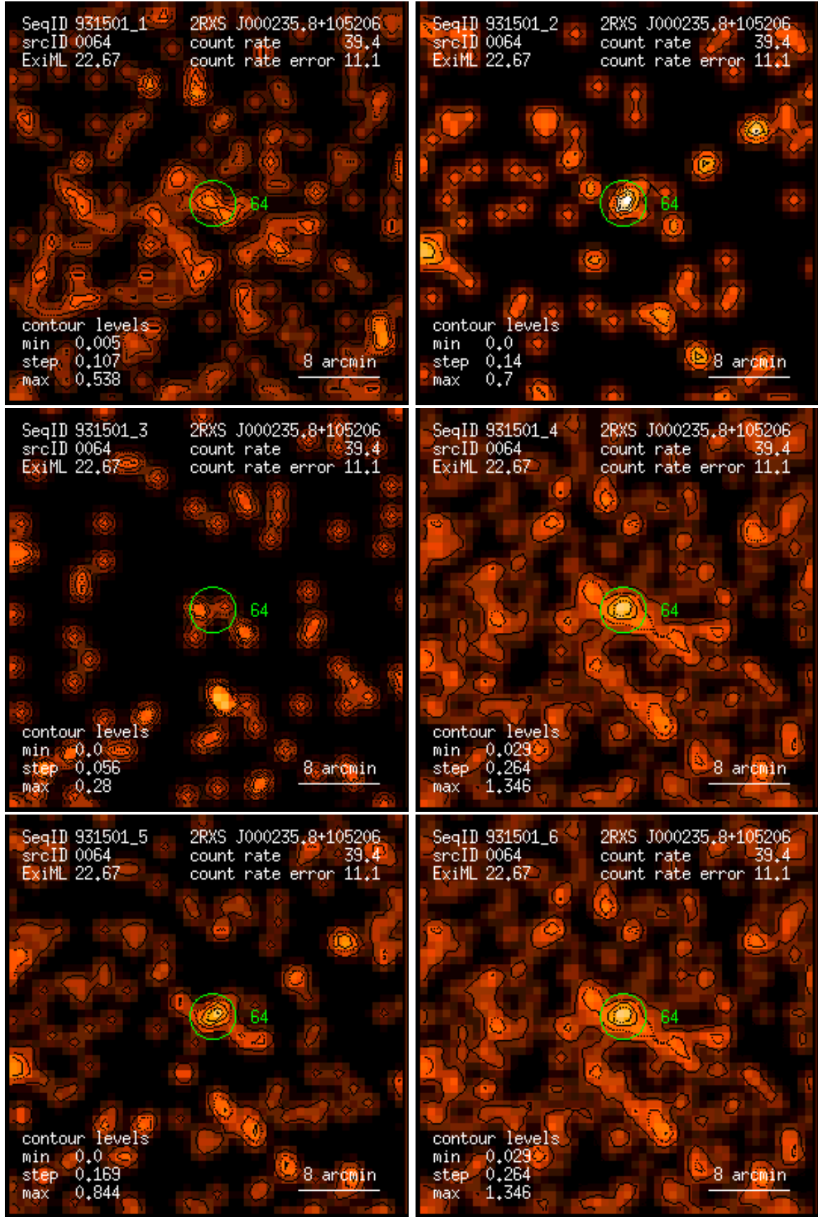
Figure 64: RASS 931501: detection 0064: band rate images, Gaussian filter: (1) PSPC channels 11 – 41, (2) 52 – 90, (3) 91 – 201, (4) 11 – 235, (5) 52 – 201, (6) 11 – 201. Broad band rates in counts/ks. Band rate contour levels in counts/ks/arcmin 2 .
