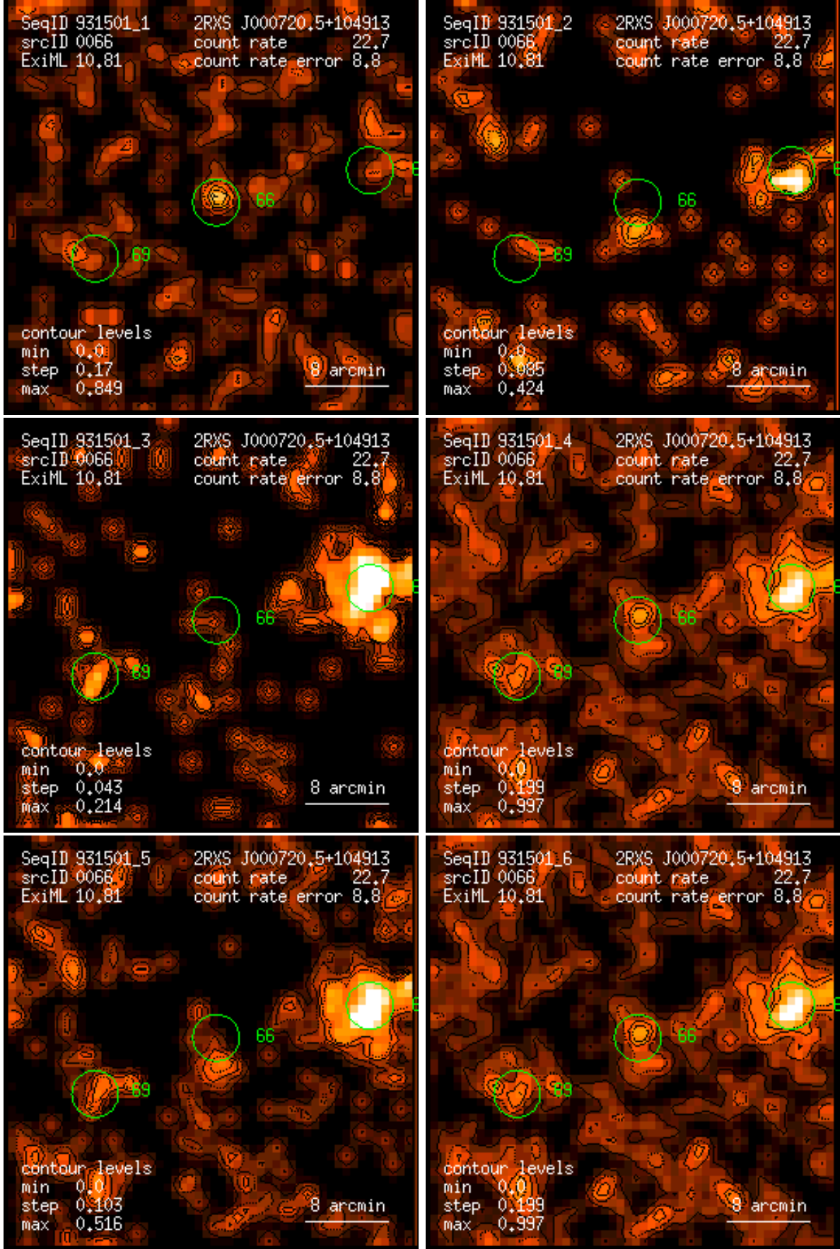
Figure 66: RASS 931501: detection 0066: band rate images, Gaussian filter: (1) PSPC channels 11 – 41, (2) 52 – 90, (3) 91 – 201, (4) 11 – 235, (5) 52 – 201, (6) 11 – 201. Broad band rates in counts/ks. Band rate contour levels in counts/ks/arcmin 2 .
