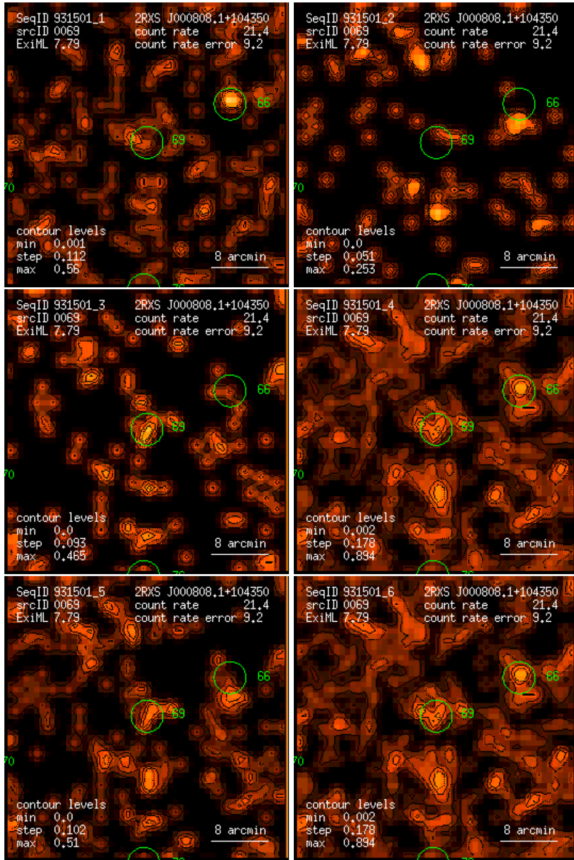
Figure 69: RASS 931501: detection 0069: band rate images, Gaussian filter: (1) PSPC channels 11 – 41, (2) 52 – 90, (3) 91 – 201, (4) 11 – 235, (5) 52 – 201, (6) 11 – 201. Broad band rates in counts/ks. Band rate contour levels in counts/ks/arcmin 2 .
