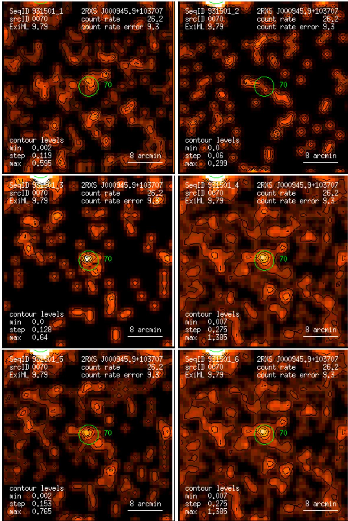
Figure 70: RASS 931501: detection 0070: band rate images, Gaussian filter: (1) PSPC channels 11 – 41, (2) 52 – 90, (3) 91 – 201, (4) 11 – 235, (5) 52 – 201, (6) 11 – 201. Broad band rates in counts/ks. Band rate contour levels in counts/ks/arcmin 2 .
