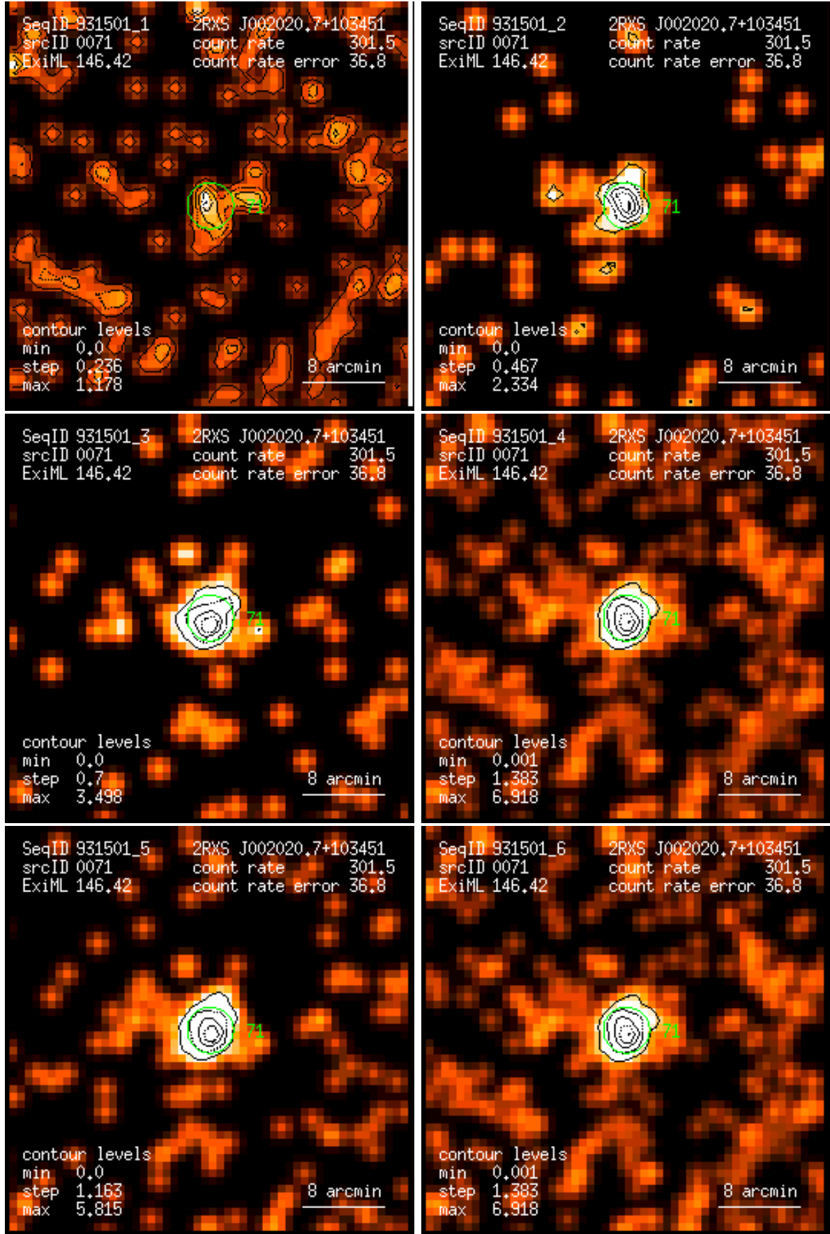
Figure 71: RASS 931501: detection 0071: band rate images, Gaussian filter: (1) PSPC channels 11 – 41, (2) 52 – 90, (3) 91 – 201, (4) 11 – 235, (5) 52 – 201, (6) 11 – 201. Broad band rates in counts/ks. Band rate contour levels in counts/ks/arcmin 2 .
