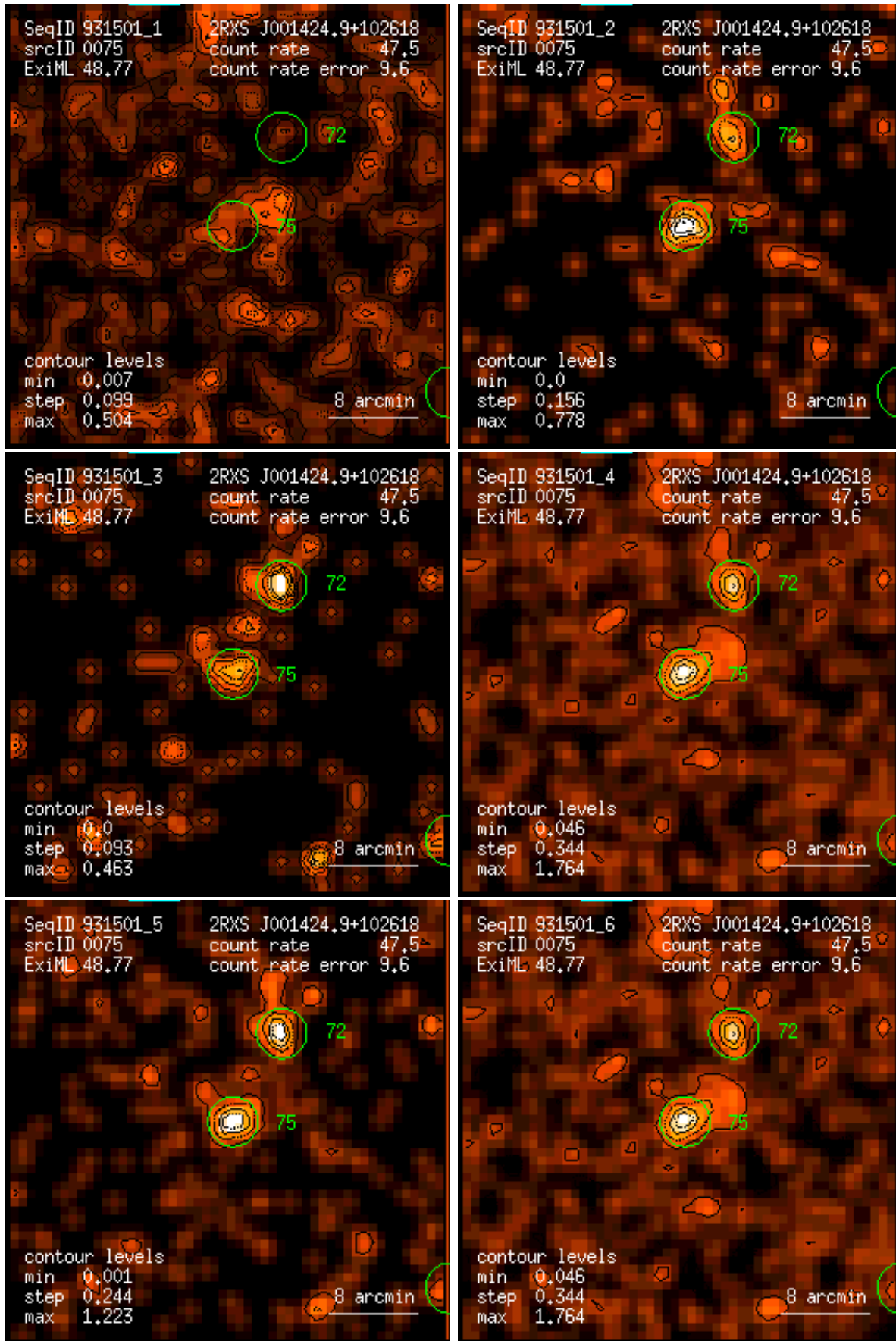
Figure 75: RASS 931501: detection 0075: band rate images, Gaussian filter: (1) PSPC channels 11 – 41, (2) 52 – 90, (3) 91 – 201, (4) 11 – 235, (5) 52 – 201, (6) 11 – 201. Broad band rates in counts/ks. Band rate contour levels in counts/ks/arcmin 2 .
