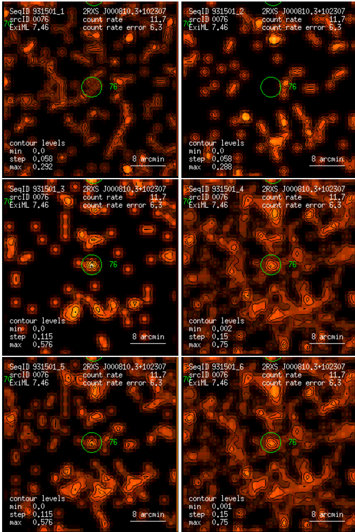
Figure 76: RASS 931501: detection 0076: band rate images, Gaussian filter: (1) PSPC channels 11 – 41, (2) 52 – 90, (3) 91 – 201, (4) 11 – 235, (5) 52 – 201, (6) 11 – 201. Broad band rates in counts/ks. Band rate contour levels in counts/ks/arcmin 2 .
