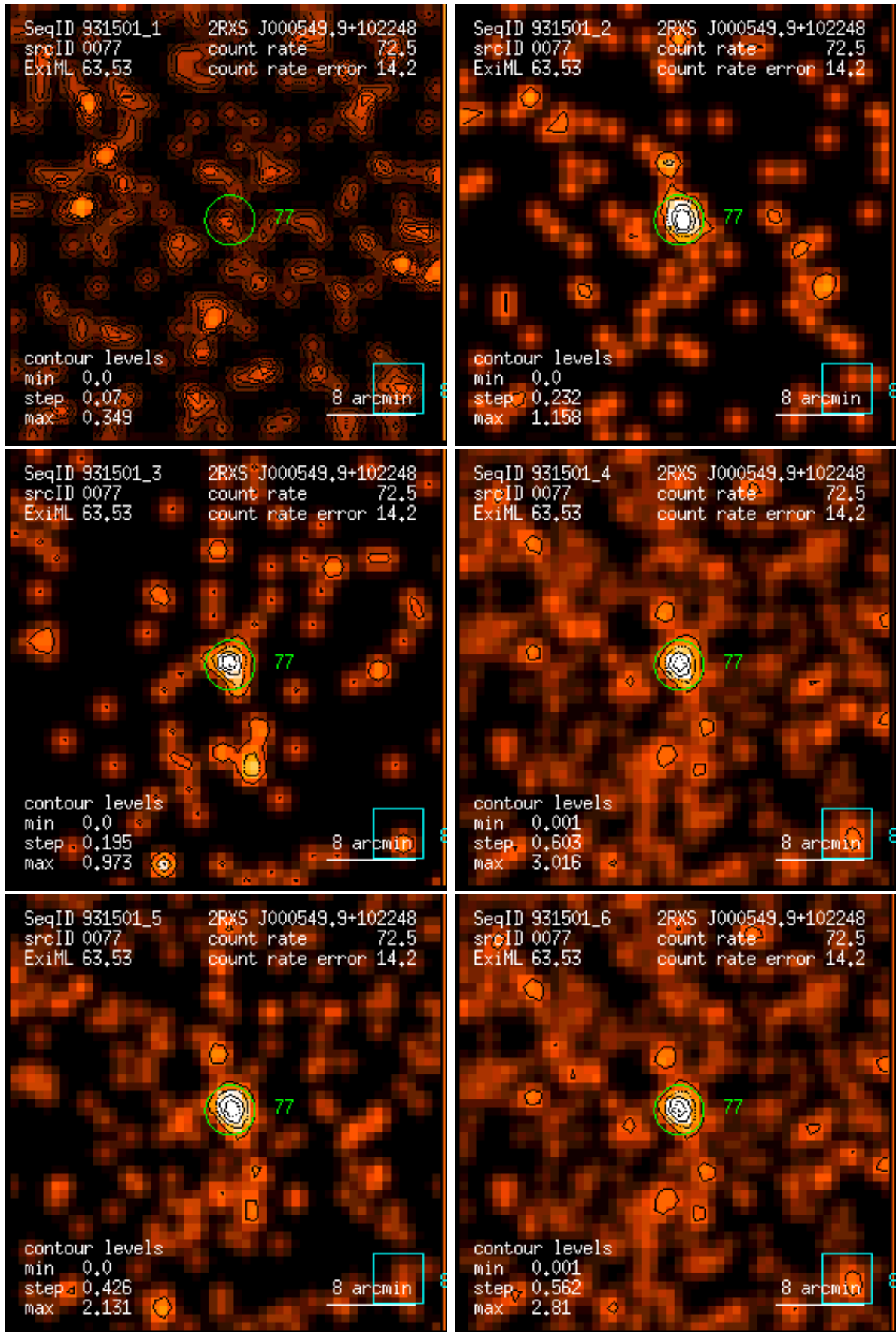
Figure 77: RASS 931501: detection 0077: band rate images, Gaussian filter: (1) PSPC channels 11 – 41, (2) 52 – 90, (3) 91 – 201, (4) 11 – 235, (5) 52 – 201, (6) 11 – 201. Broad band rates in counts/ks. Band rate contour levels in counts/ks/arcmin 2 .
