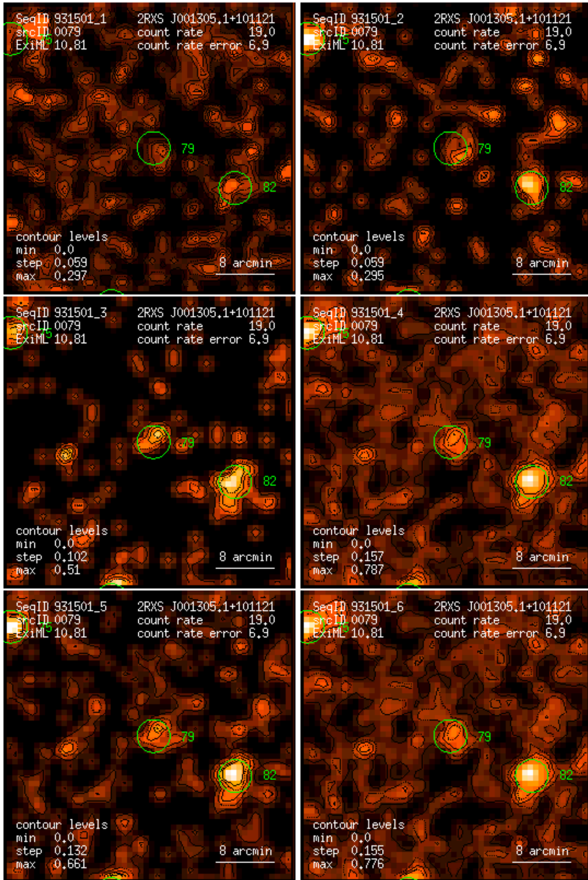
Figure 79: RASS 931501: detection 0079: band rate images, Gaussian filter: (1) PSPC channels 11 – 41, (2) 52 – 90, (3) 91 – 201, (4) 11 – 235, (5) 52 – 201, (6) 11 – 201. Broad band rates in counts/ks. Band rate contour levels in counts/ks/arcmin 2 .
