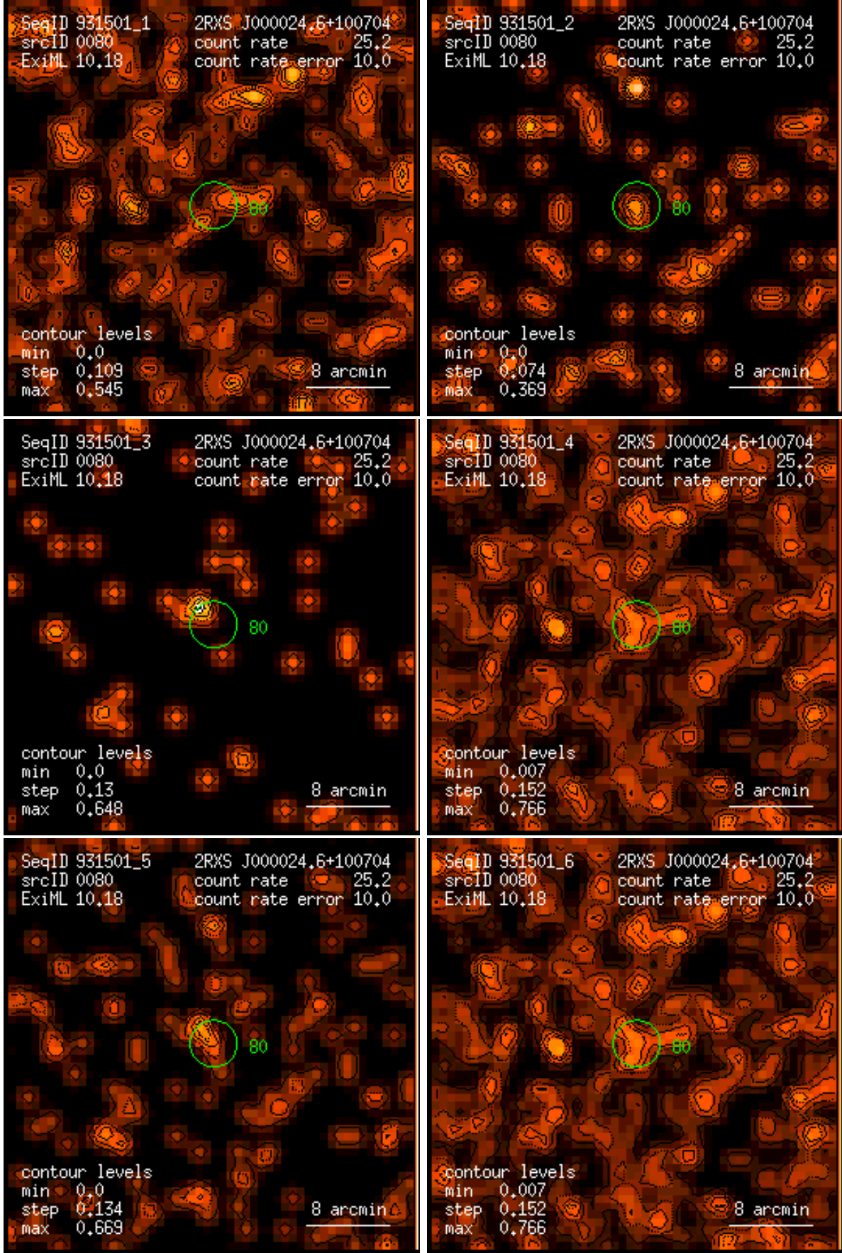
Figure 80: RASS 931501: detection 0080: band rate images, Gaussian filter: (1) PSPC channels 11 – 41, (2) 52 – 90, (3) 91 – 201, (4) 11 – 235, (5) 52 – 201, (6) 11 – 201. Broad band rates in counts/ks. Band rate contour levels in counts/ks/arcmin 2 .
