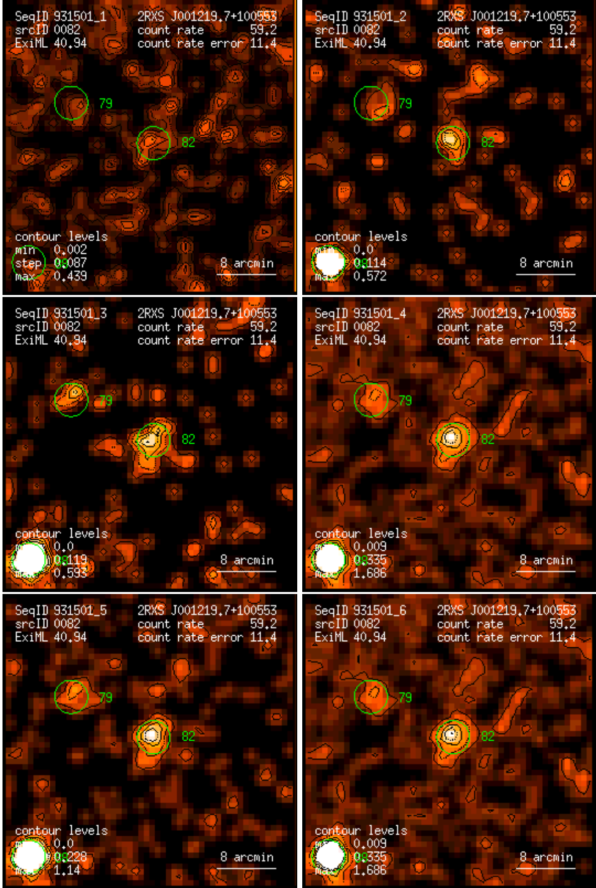
Figure 82: RASS 931501: detection 0082: band rate images, Gaussian filter: (1) PSPC channels 11 – 41, (2) 52 – 90, (3) 91 – 201, (4) 11 – 235, (5) 52 – 201, (6) 11 – 201. Broad band rates in counts/ks. Band rate contour levels in counts/ks/arcmin 2 .
