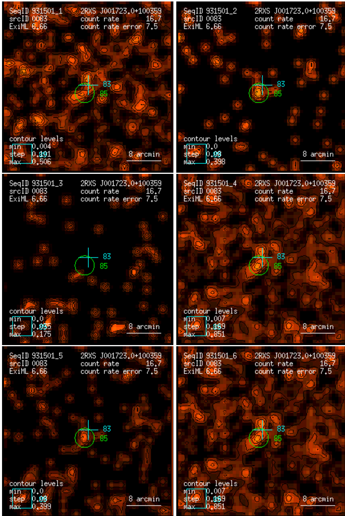
Figure 83: RASS 931501: detection 0083: band rate images, Gaussian filter: (1) PSPC channels 11 – 41, (2) 52 – 90, (3) 91 – 201, (4) 11 – 235, (5) 52 – 201, (6) 11 – 201. Broad band rates in counts/ks. Band rate contour levels in counts/ks/arcmin 2 .
