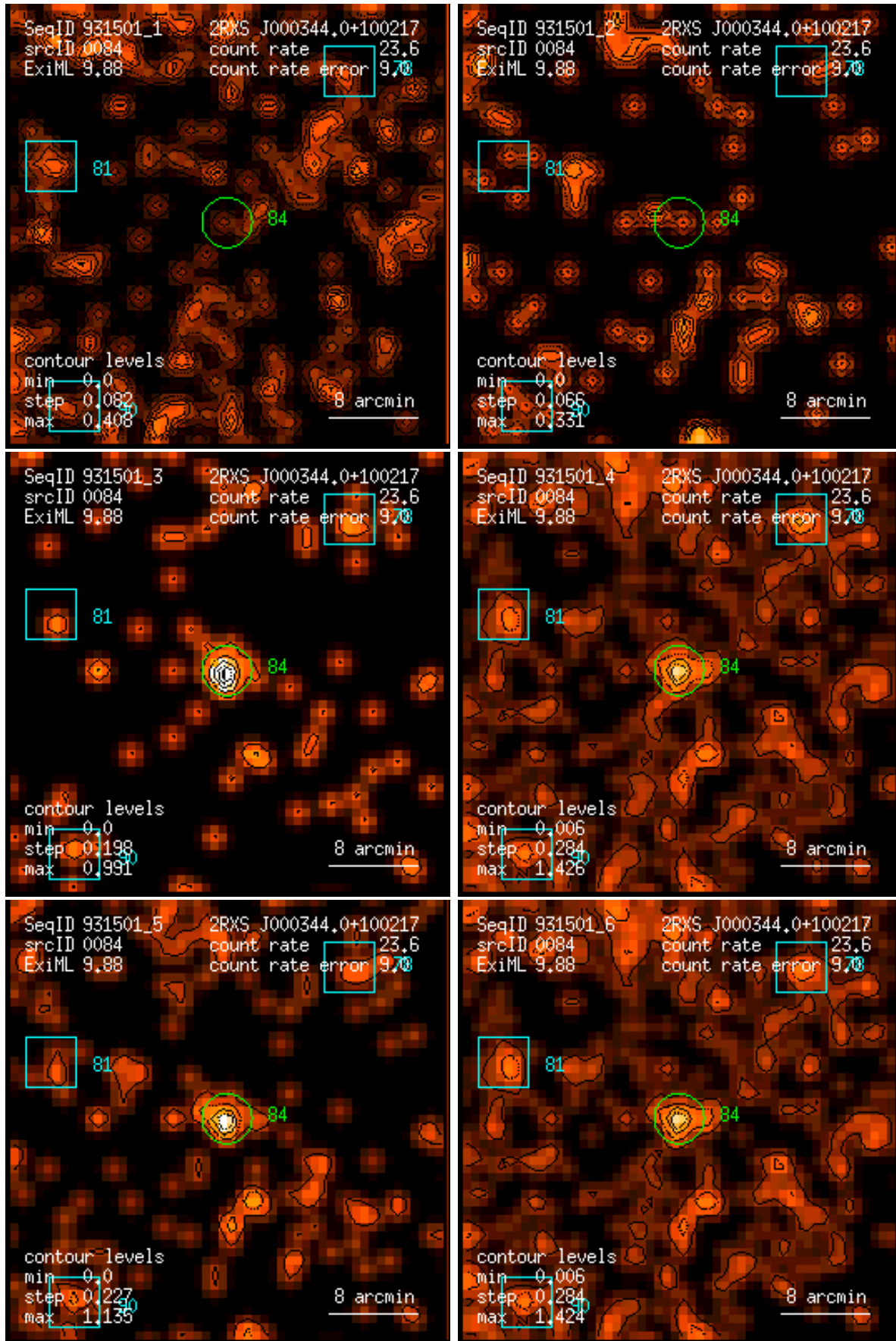
Figure 84: RASS 931501: detection 0084: band rate images, Gaussian filter: (1) PSPC channels 11 – 41, (2) 52 – 90, (3) 91 – 201, (4) 11 – 235, (5) 52 – 201, (6) 11 – 201. Broad band rates in counts/ks. Band rate contour levels in counts/ks/arcmin 2 .
