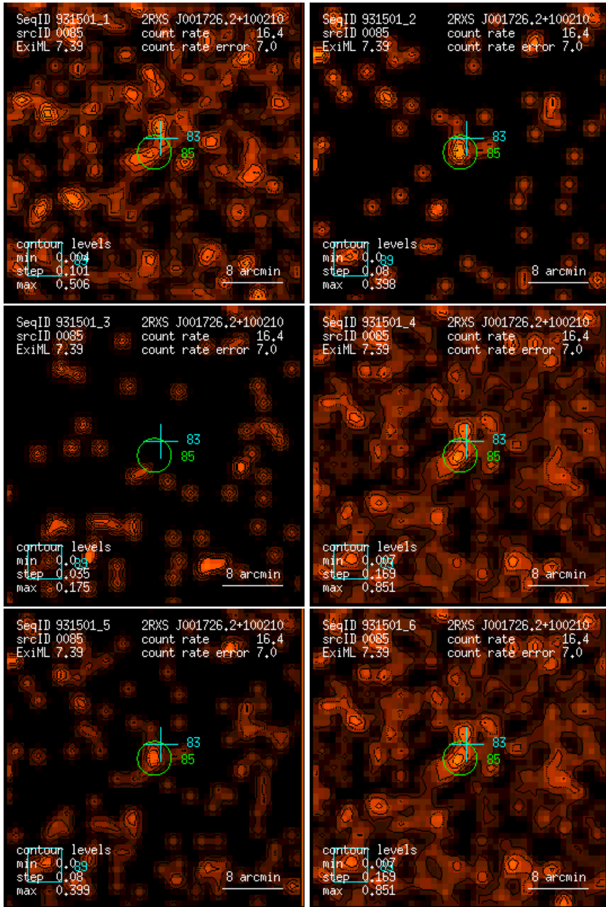
Figure 85: RASS 931501: detection 0085: band rate images, Gaussian filter: (1) PSPC channels 11 – 41, (2) 52 – 90, (3) 91 – 201, (4) 11 – 235, (5) 52 – 201, (6) 11 – 201. Broad band rates in counts/ks. Band rate contour levels in counts/ks/arcmin 2 .
