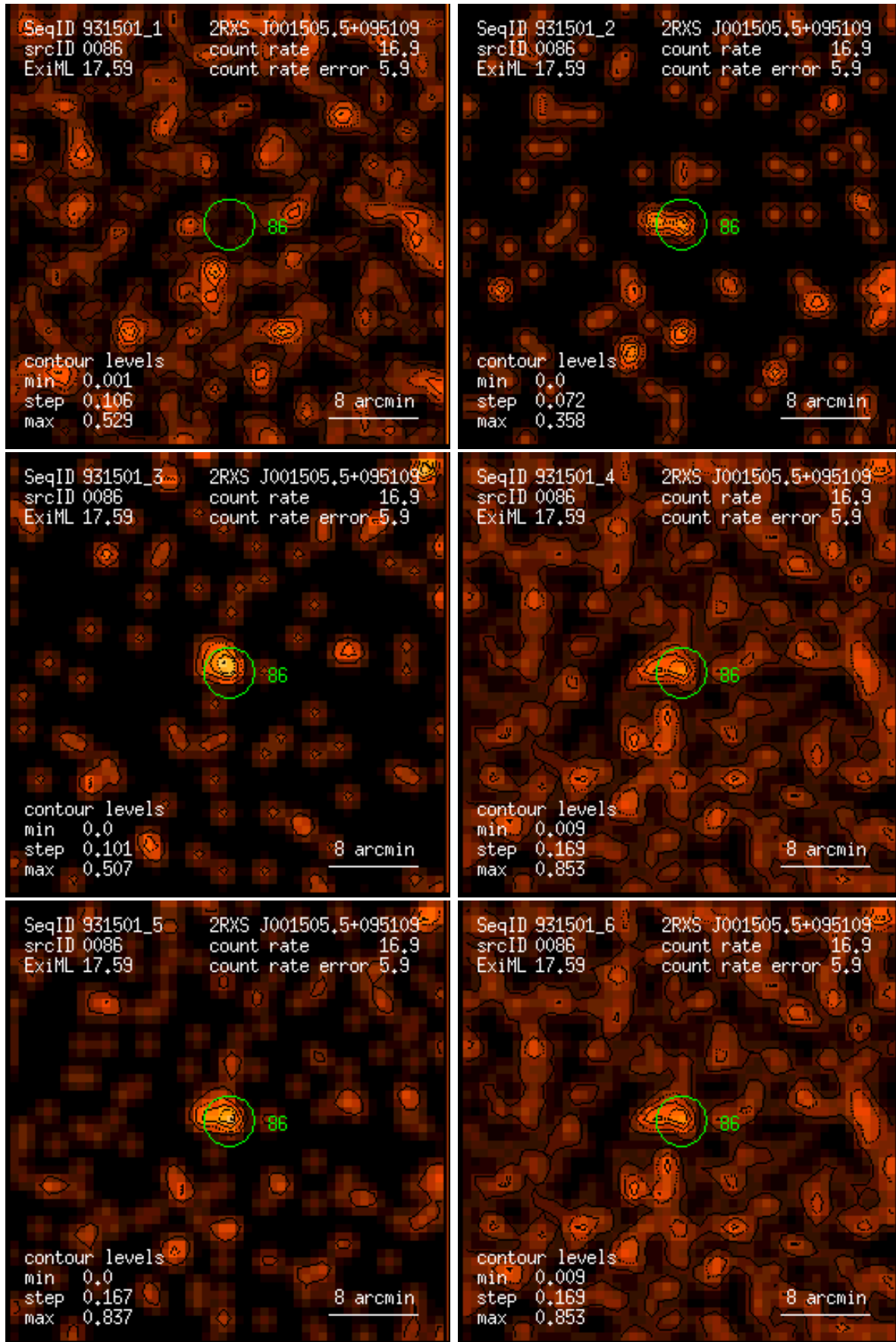
Figure 86: RASS 931501: detection 0086: band rate images, Gaussian filter: (1) PSPC channels 11 – 41, (2) 52 – 90, (3) 91 – 201, (4) 11 – 235, (5) 52 – 201, (6) 11 – 201. Broad band rates in counts/ks. Band rate contour levels in counts/ks/arcmin 2 .
