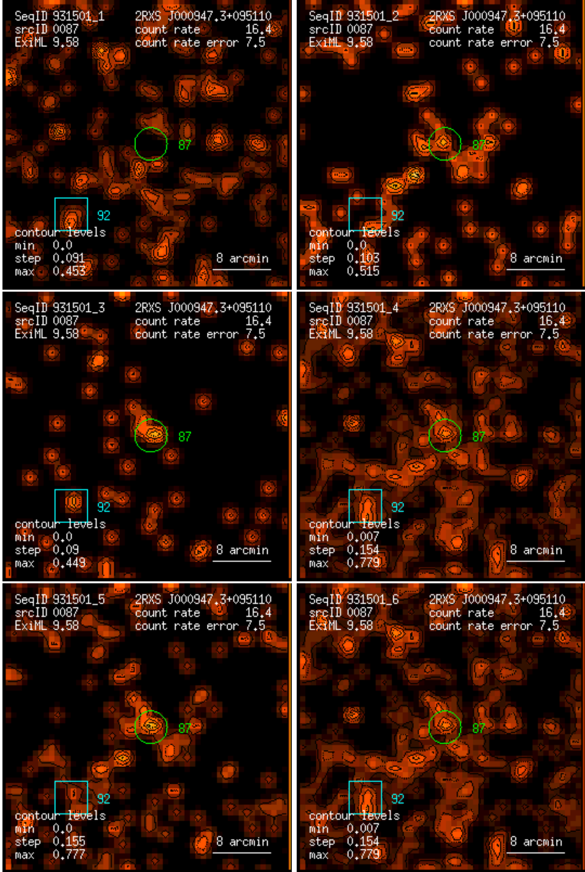
Figure 87: RASS 931501: detection 0087: band rate images, Gaussian filter: (1) PSPC channels 11 – 41, (2) 52 – 90, (3) 91 – 201, (4) 11 – 235, (5) 52 – 201, (6) 11 – 201. Broad band rates in counts/ks. Band rate contour levels in counts/ks/arcmin 2 .
