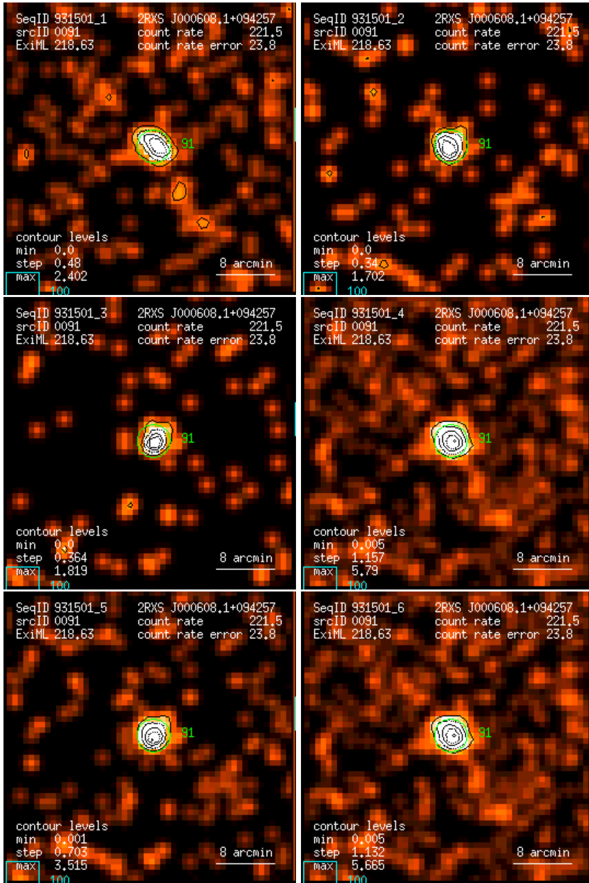
Figure 91: RASS 931501: detection 0091: band rate images, Gaussian filter: (1) PSPC channels 11 – 41, (2) 52 – 90, (3) 91 – 201, (4) 11 – 235, (5) 52 – 201, (6) 11 – 201. Broad band rates in counts/ks. Band rate contour levels in counts/ks/arcmin 2 .
