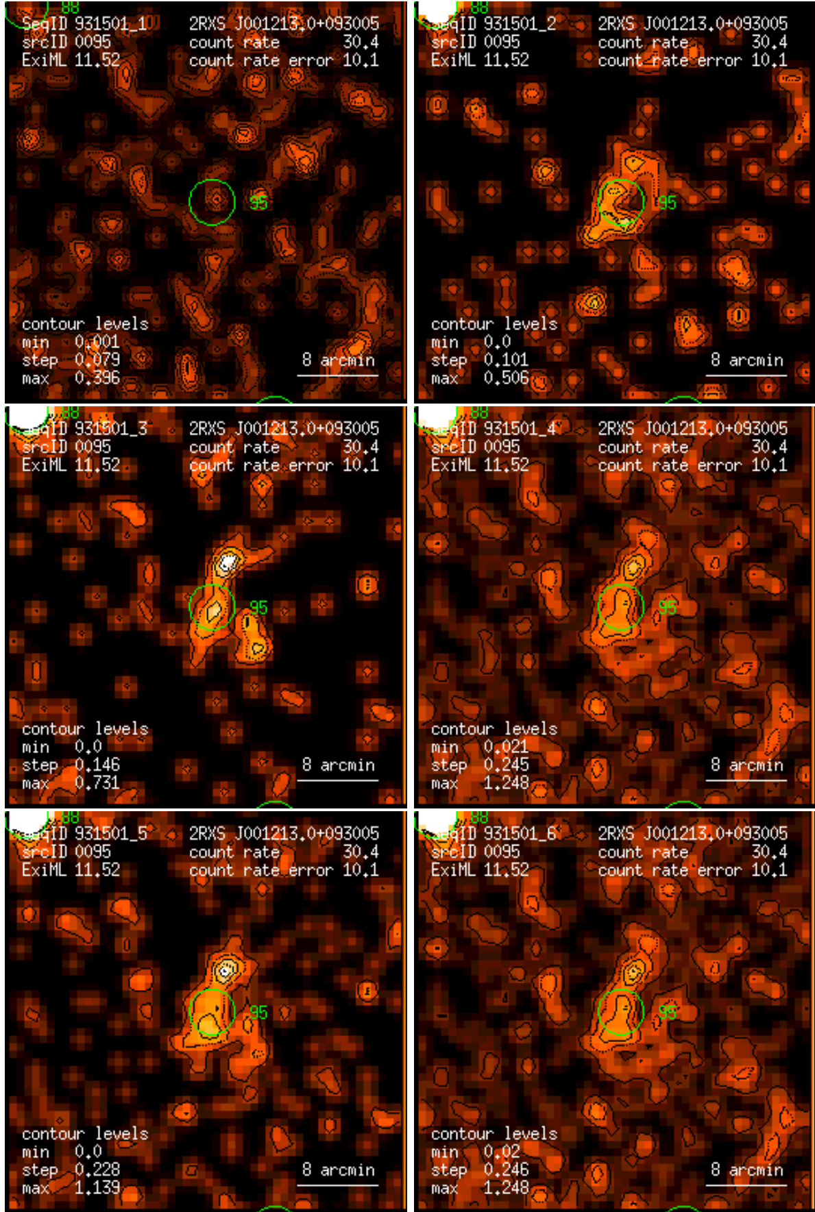
Figure 95: RASS 931501: detection 0095: band rate images, Gaussian filter: (1) PSPC channels 11 – 41, (2) 52 – 90, (3) 91 – 201, (4) 11 – 235, (5) 52 – 201, (6) 11 – 201. Broad band rates in counts/ks. Band rate contour levels in counts/ks/arcmin 2 .
