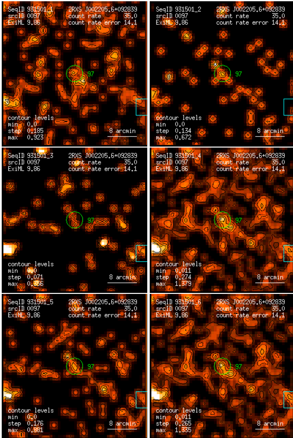
Figure 97: RASS 931501: detection 0097: band rate images, Gaussian filter: (1) PSPC channels 11 – 41, (2) 52 – 90, (3) 91 – 201, (4) 11 – 235, (5) 52 – 201, (6) 11 – 201. Broad band rates in counts/ks. Band rate contour levels in counts/ks/arcmin 2 .
