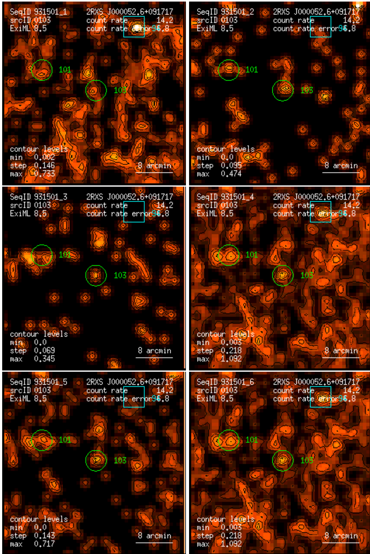
Figure 103: RASS 931501: detection 0103: band rate images, Gaussian filter: (1) PSPC channels 11 – 41, (2) 52 – 90, (3) 91 – 201, (4) 11 – 235, (5) 52 – 201, (6) 11 – 201. Broad band rates in counts/ks. Band rate contour levels in counts/ks/arcmin 2 .
