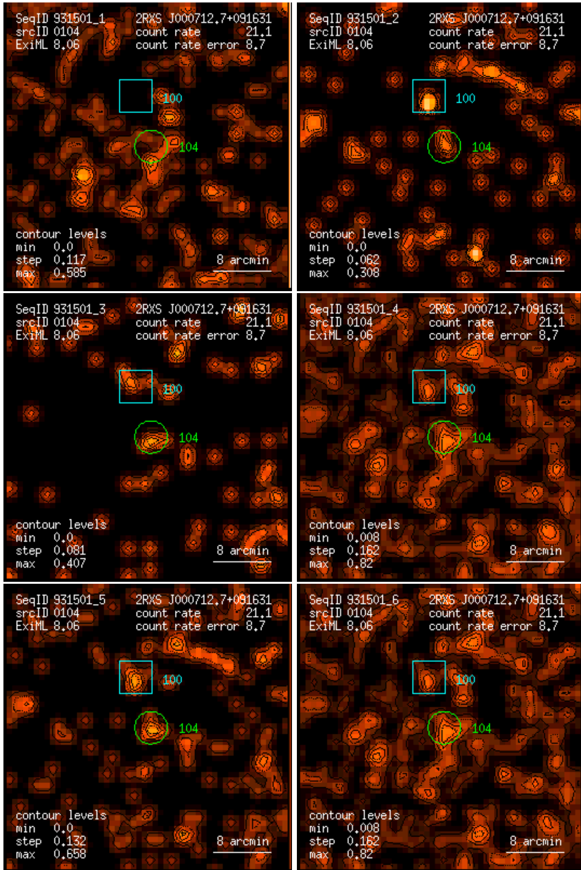
Figure 104: RASS 931501: detection 0104: band rate images, Gaussian filter: (1) PSPC channels 11 – 41, (2) 52 – 90, (3) 91 – 201, (4) 11 – 235, (5) 52 – 201, (6) 11 – 201. Broad band rates in counts/ks. Band rate contour levels in counts/ks/arcmin 2 .
