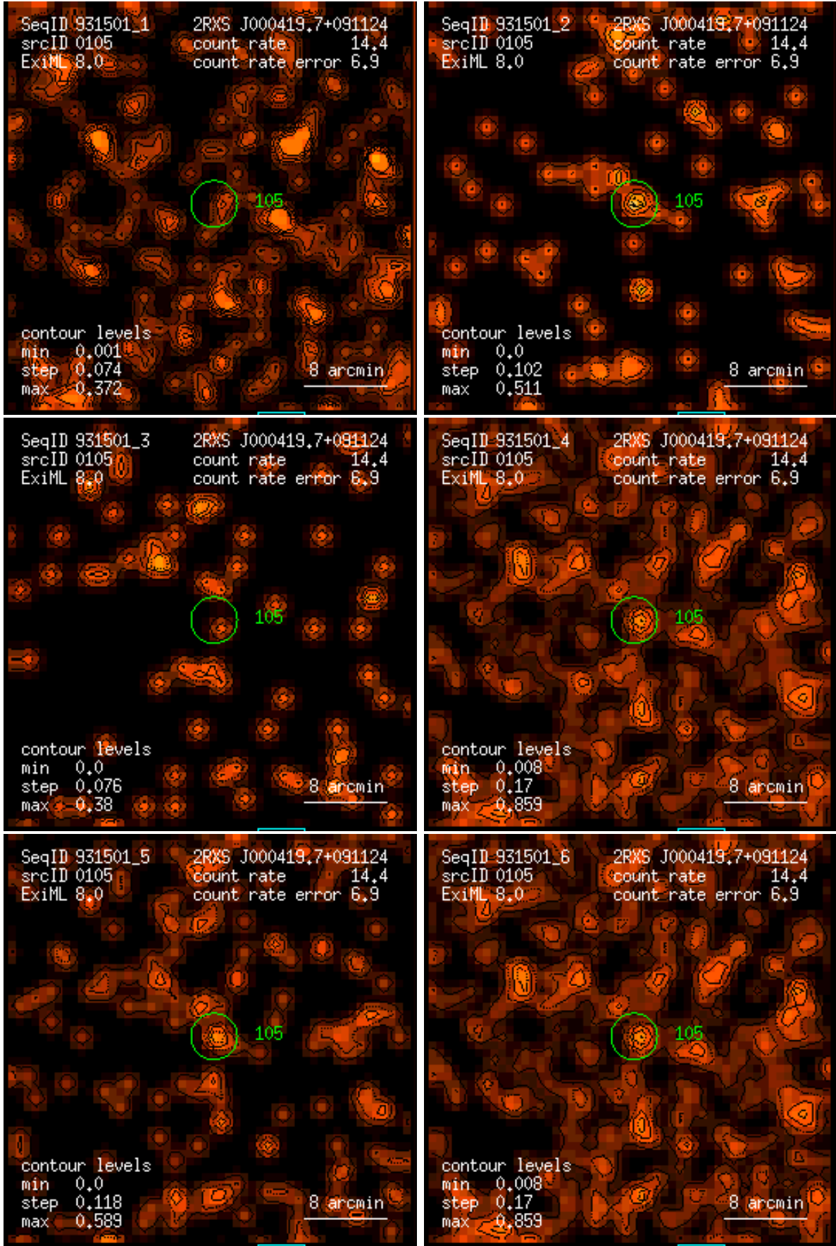
Figure 105: RASS 931501: detection 0105: band rate images, Gaussian filter: (1) PSPC channels 11 – 41, (2) 52 – 90, (3) 91 – 201, (4) 11 – 235, (5) 52 – 201, (6) 11 – 201. Broad band rates in counts/ks. Band rate contour levels in counts/ks/arcmin 2 .
