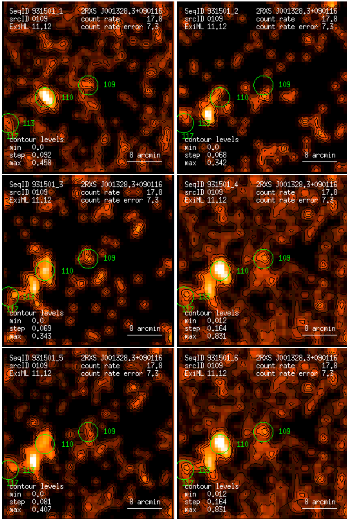
Figure 109: RASS 931501: detection 0109: band rate images, Gaussian filter: (1) PSPC channels 11 – 41, (2) 52 – 90, (3) 91 – 201, (4) 11 – 235, (5) 52 – 201, (6) 11 – 201. Broad band rates in counts/ks. Band rate contour levels in counts/ks/arcmin 2 .
