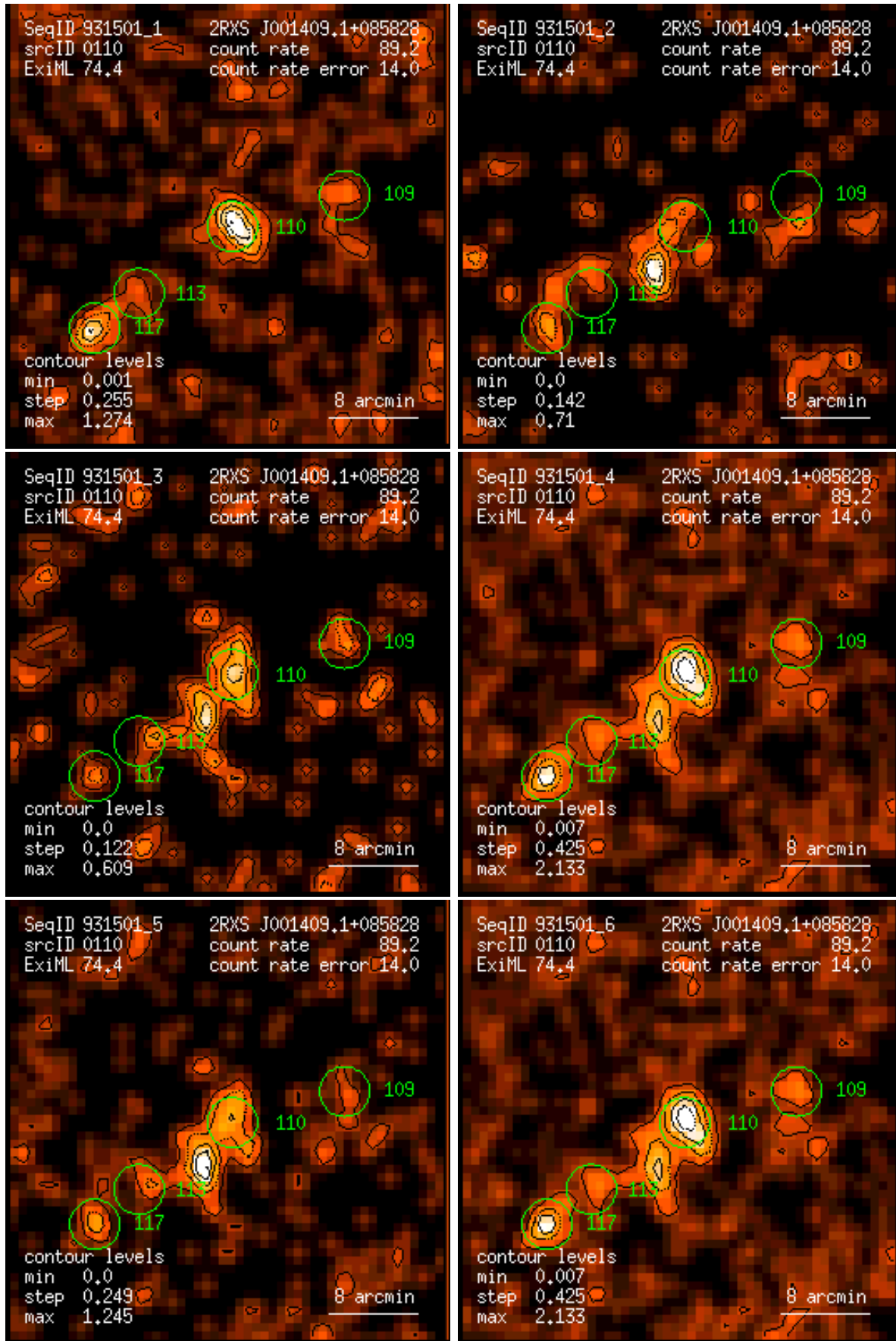
Figure 110: RASS 931501: detection 0110: band rate images, Gaussian filter: (1) PSPC channels 11 – 41, (2) 52 – 90, (3) 91 – 201, (4) 11 – 235, (5) 52 – 201, (6) 11 – 201. Broad band rates in counts/ks. Band rate contour levels in counts/ks/arcmin 2 .
