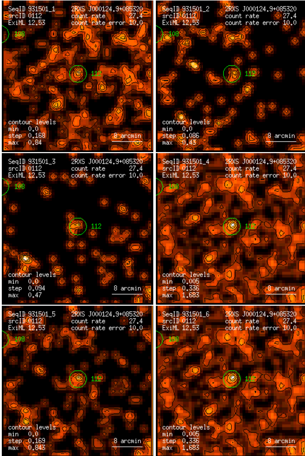
Figure 112: RASS 931501: detection 0112: band rate images, Gaussian filter: (1) PSPC channels 11 – 41, (2) 52 – 90, (3) 91 – 201, (4) 11 – 235, (5) 52 – 201, (6) 11 – 201. Broad band rates in counts/ks. Band rate contour levels in counts/ks/arcmin 2 .
