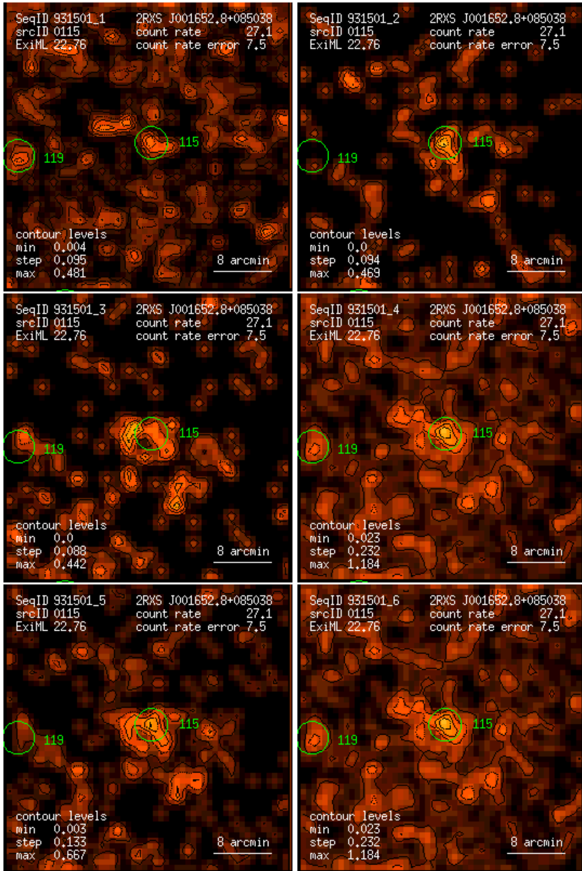
Figure 115: RASS 931501: detection 0115: band rate images, Gaussian filter: (1) PSPC channels 11 – 41, (2) 52 – 90, (3) 91 – 201, (4) 11 – 235, (5) 52 – 201, (6) 11 – 201. Broad band rates in counts/ks. Band rate contour levels in counts/ks/arcmin 2 .
