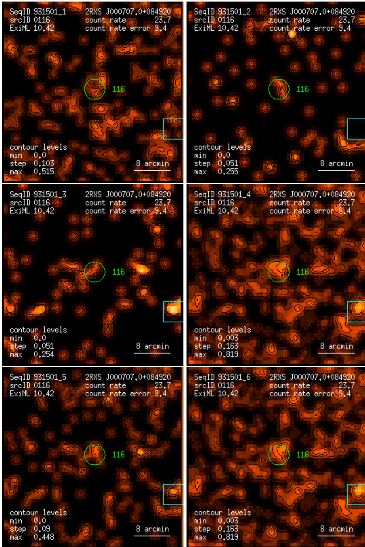
Figure 116: RASS 931501: detection 0116: band rate images, Gaussian filter: (1) PSPC channels 11 – 41, (2) 52 – 90, (3) 91 – 201, (4) 11 – 235, (5) 52 – 201, (6) 11 – 201. Broad band rates in counts/ks. Band rate contour levels in counts/ks/arcmin 2 .
