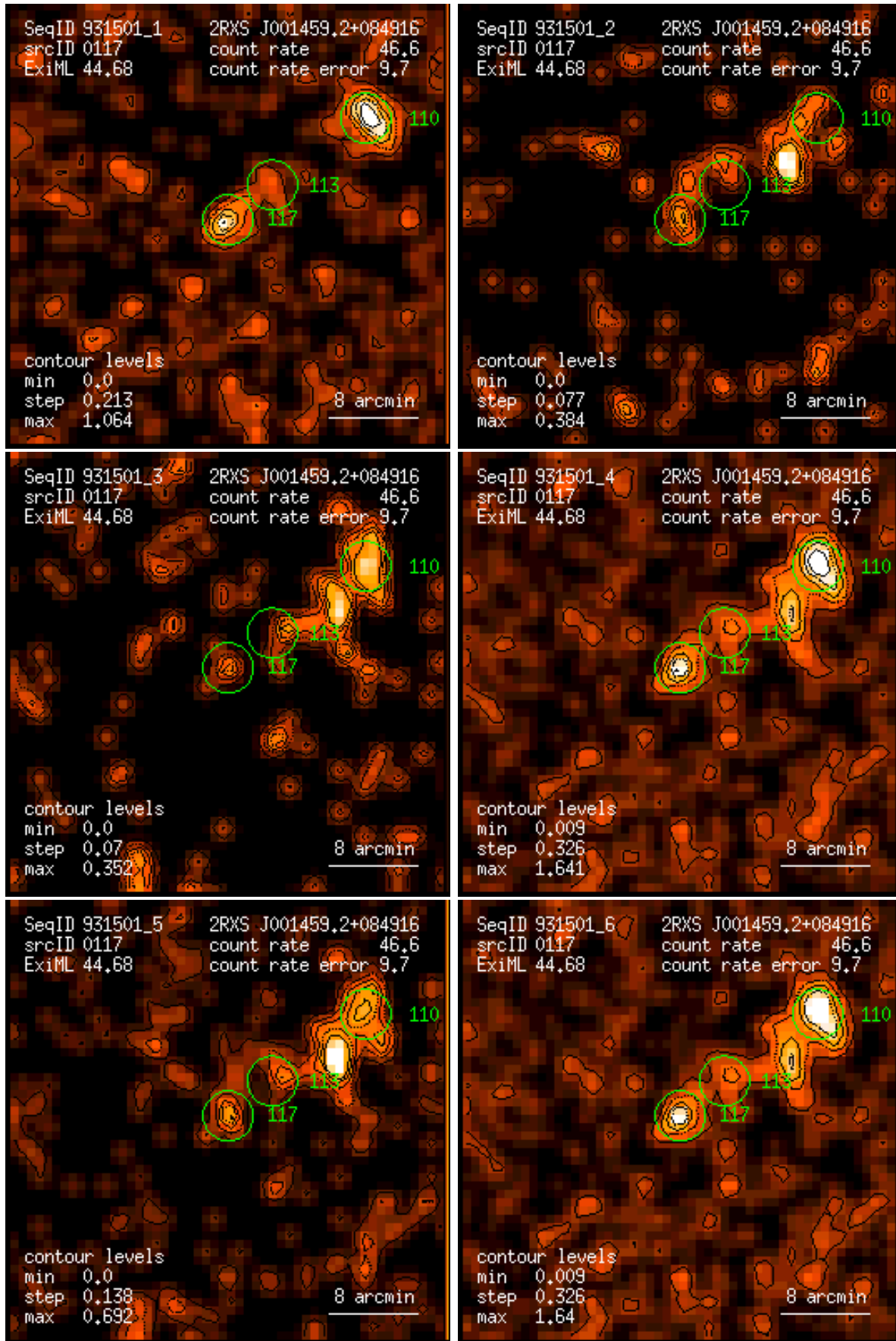
Figure 117: RASS 931501: detection 0117: band rate images, Gaussian filter: (1) PSPC channels 11 – 41, (2) 52 – 90, (3) 91 – 201, (4) 11 – 235, (5) 52 – 201, (6) 11 – 201. Broad band rates in counts/ks. Band rate contour levels in counts/ks/arcmin 2 .
