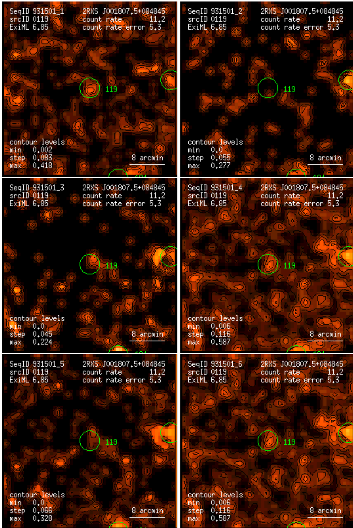
Figure 119: RASS 931501: detection 0119: band rate images, Gaussian filter: (1) PSPC channels 11 – 41, (2) 52 – 90, (3) 91 – 201, (4) 11 – 235, (5) 52 – 201, (6) 11 – 201. Broad band rates in counts/ks. Band rate contour levels in counts/ks/arcmin 2 .
