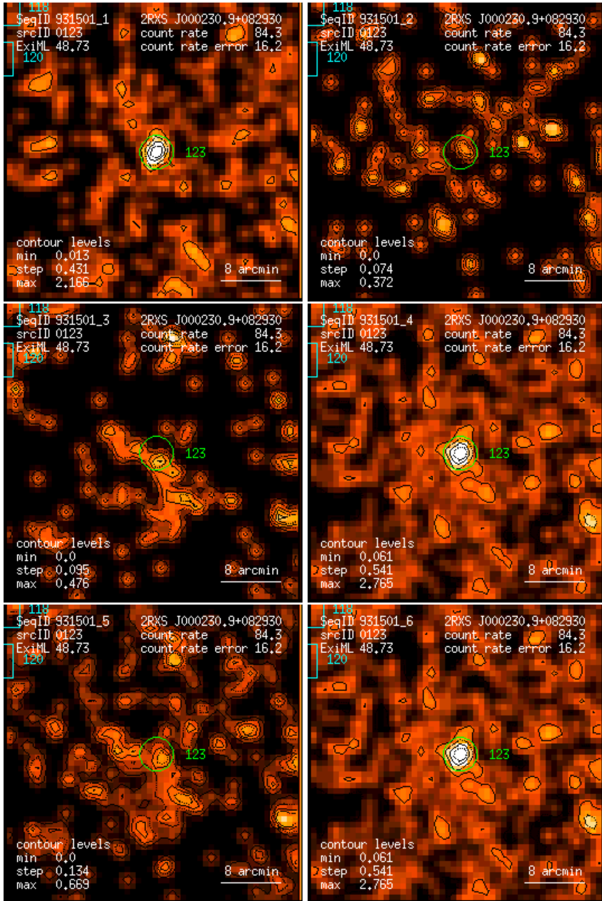
Figure 123: RASS 931501: detection 0123: band rate images, Gaussian filter: (1) PSPC channels 11 – 41, (2) 52 – 90, (3) 91 – 201, (4) 11 – 235, (5) 52 – 201, (6) 11 – 201. Broad band rates in counts/ks. Band rate contour levels in counts/ks/arcmin 2 .
