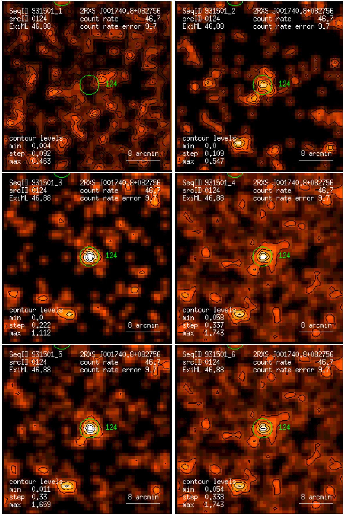
Figure 124: RASS 931501: detection 0124: band rate images, Gaussian filter: (1) PSPC channels 11 – 41, (2) 52 – 90, (3) 91 – 201, (4) 11 – 235, (5) 52 – 201, (6) 11 – 201. Broad band rates in counts/ks. Band rate contour levels in counts/ks/arcmin 2 .
