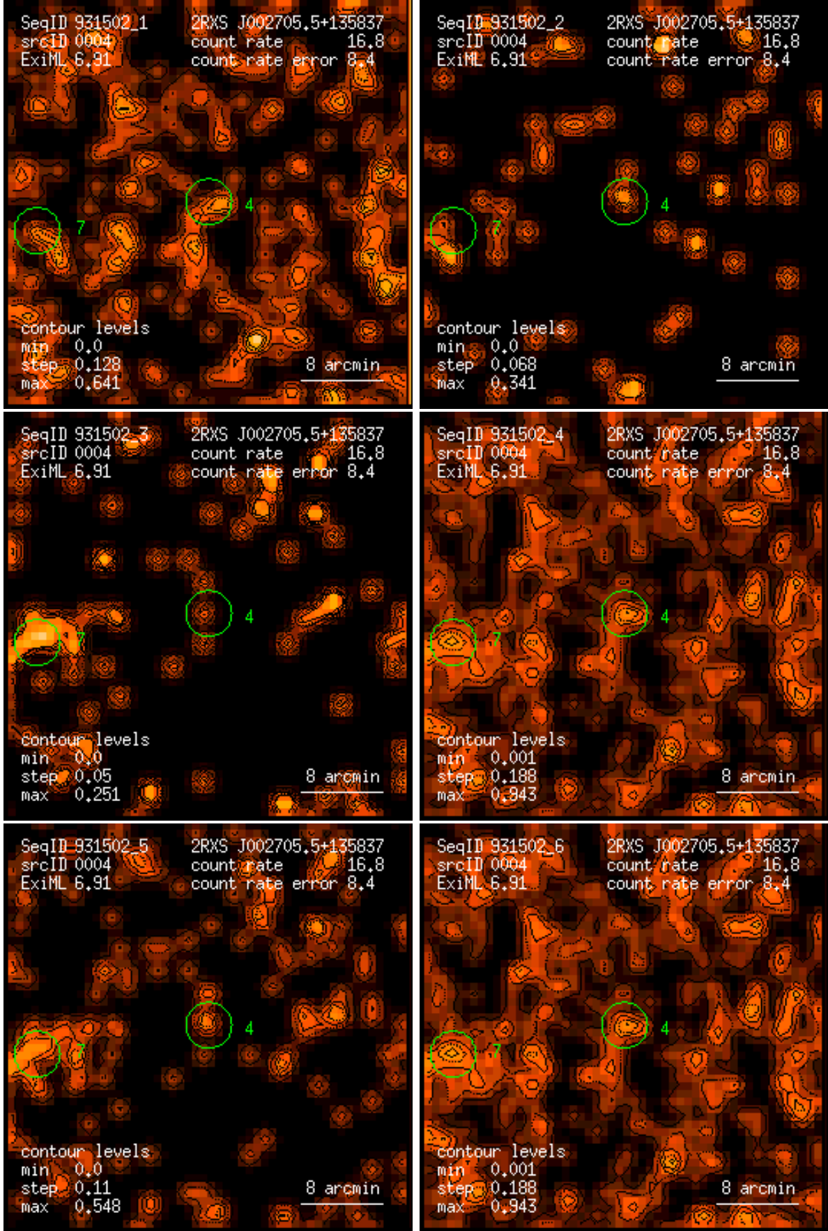
Figure 4: RASS 931502: detection 0004: band rate images, Gaussian filter: (1) PSPC channels 11 – 41, (2) 52 – 90, (3) 91 – 201, (4) 11 – 235, (5) 52 – 201, (6) 11 – 201. Broad band rates in counts/ks. Band rate contour levels in counts/ks/arcmin 2 .
