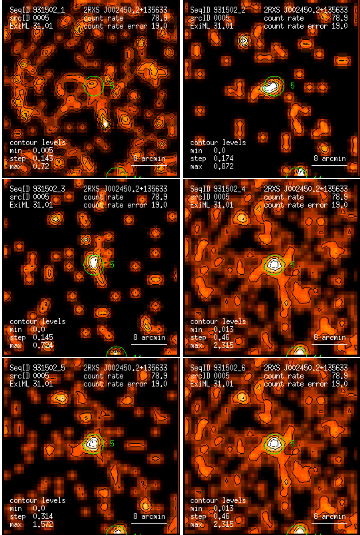
Figure 5: RASS 931502: detection 0005: band rate images, Gaussian filter: (1) PSPC channels 11 – 41, (2) 52 – 90, (3) 91 – 201, (4) 11 – 235, (5) 52 – 201, (6) 11 – 201. Broad band rates in counts/ks. Band rate contour levels in counts/ks/arcmin 2 .
