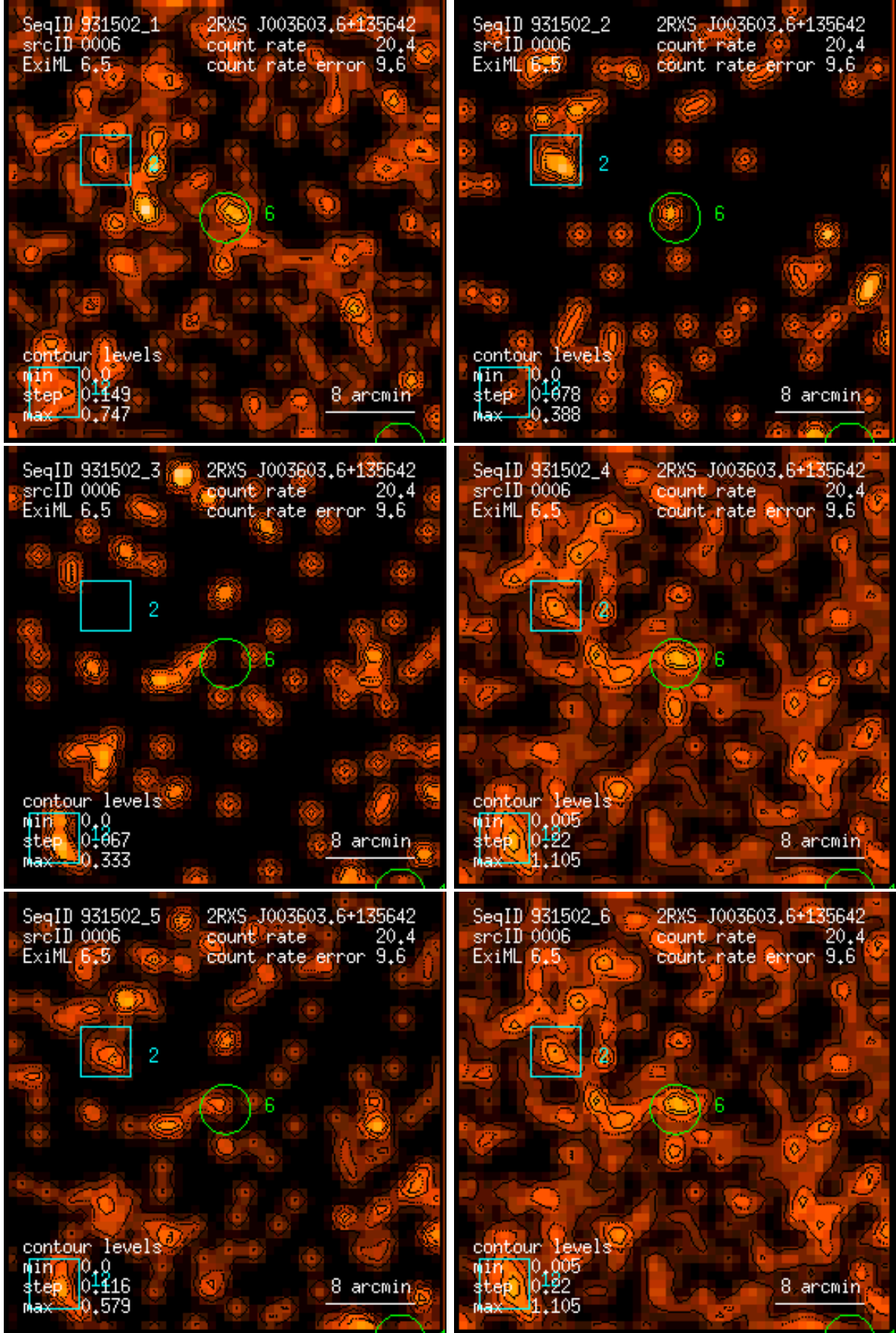
Figure 6: RASS 931502: detection 0006: band rate images, Gaussian filter: (1) PSPC channels 11 – 41, (2) 52 – 90, (3) 91 – 201, (4) 11 – 235, (5) 52 – 201, (6) 11 – 201. Broad band rates in counts/ks. Band rate contour levels in counts/ks/arcmin 2 .
