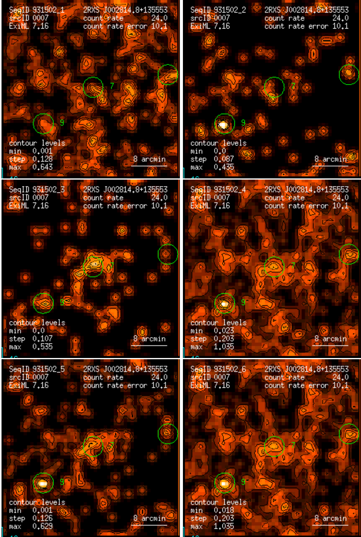
Figure 7: RASS 931502: detection 0007: band rate images, Gaussian filter: (1) PSPC channels 11 – 41, (2) 52 – 90, (3) 91 – 201, (4) 11 – 235, (5) 52 – 201, (6) 11 – 201. Broad band rates in counts/ks. Band rate contour levels in counts/ks/arcmin 2 .
