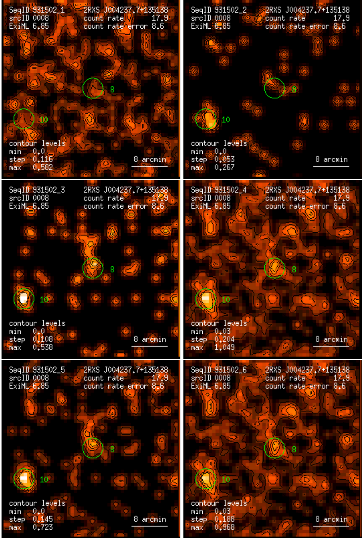
Figure 8: RASS 931502: detection 0008: band rate images, Gaussian filter: (1) PSPC channels 11 – 41, (2) 52 – 90, (3) 91 – 201, (4) 11 – 235, (5) 52 – 201, (6) 11 – 201. Broad band rates in counts/ks. Band rate contour levels in counts/ks/arcmin 2 .
