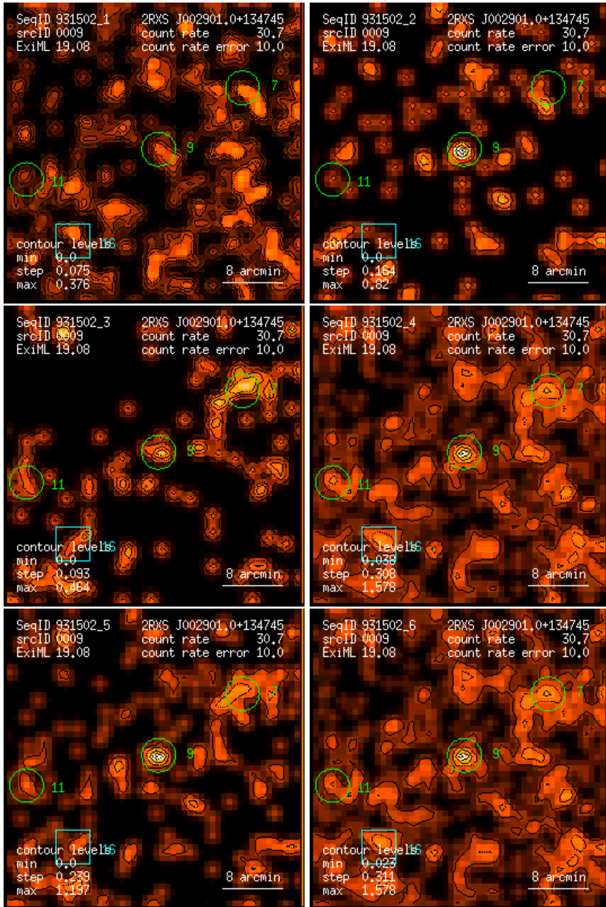
Figure 9: RASS 931502: detection 0009: band rate images, Gaussian filter: (1) PSPC channels 11 – 41, (2) 52 – 90, (3) 91 – 201, (4) 11 – 235, (5) 52 – 201, (6) 11 – 201. Broad band rates in counts/ks. Band rate contour levels in counts/ks/arcmin 2 .
