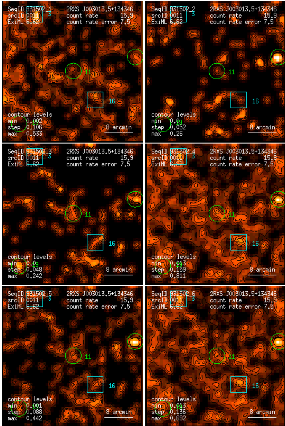
Figure 11: RASS 931502: detection 0011: band rate images, Gaussian filter: (1) PSPC channels 11 – 41, (2) 52 – 90, (3) 91 – 201, (4) 11 – 235, (5) 52 – 201, (6) 11 – 201. Broad band rates in counts/ks. Band rate contour levels in counts/ks/arcmin 2 .
