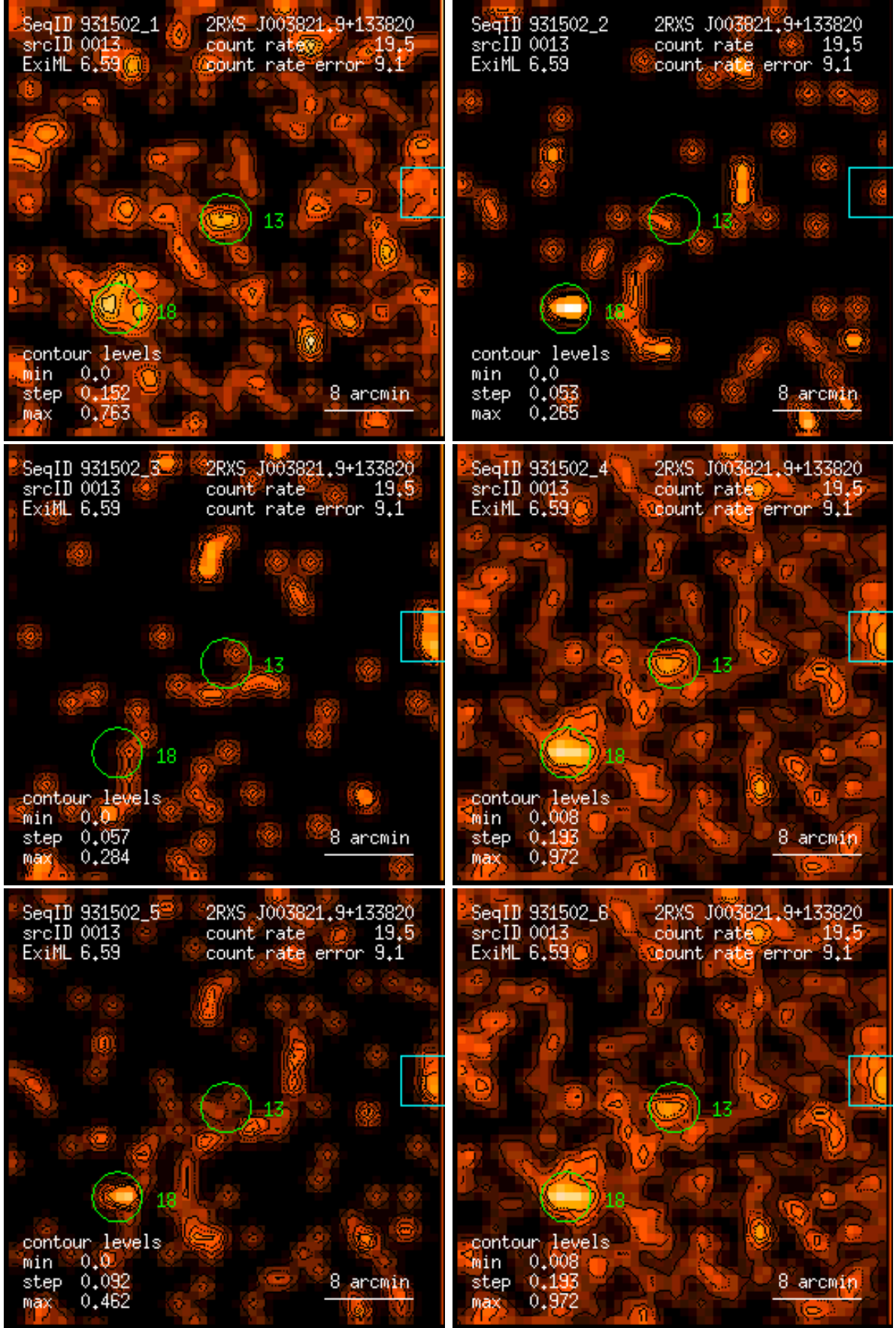
Figure 13: RASS 931502: detection 0013: band rate images, Gaussian filter: (1) PSPC channels 11 – 41, (2) 52 – 90, (3) 91 – 201, (4) 11 – 235, (5) 52 – 201, (6) 11 – 201. Broad band rates in counts/ks. Band rate contour levels in counts/ks/arcmin 2 .
