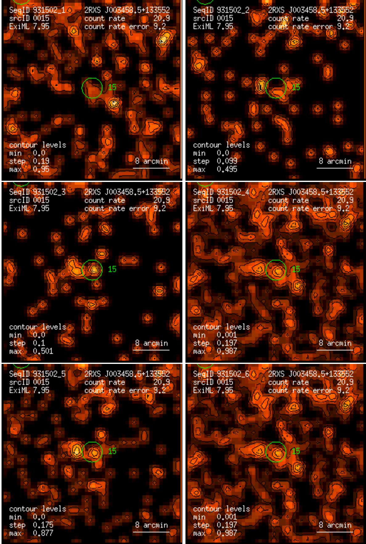
Figure 15: RASS 931502: detection 0015: band rate images, Gaussian filter: (1) PSPC channels 11 – 41, (2) 52 – 90, (3) 91 – 201, (4) 11 – 235, (5) 52 – 201, (6) 11 – 201. Broad band rates in counts/ks. Band rate contour levels in counts/ks/arcmin 2 .
