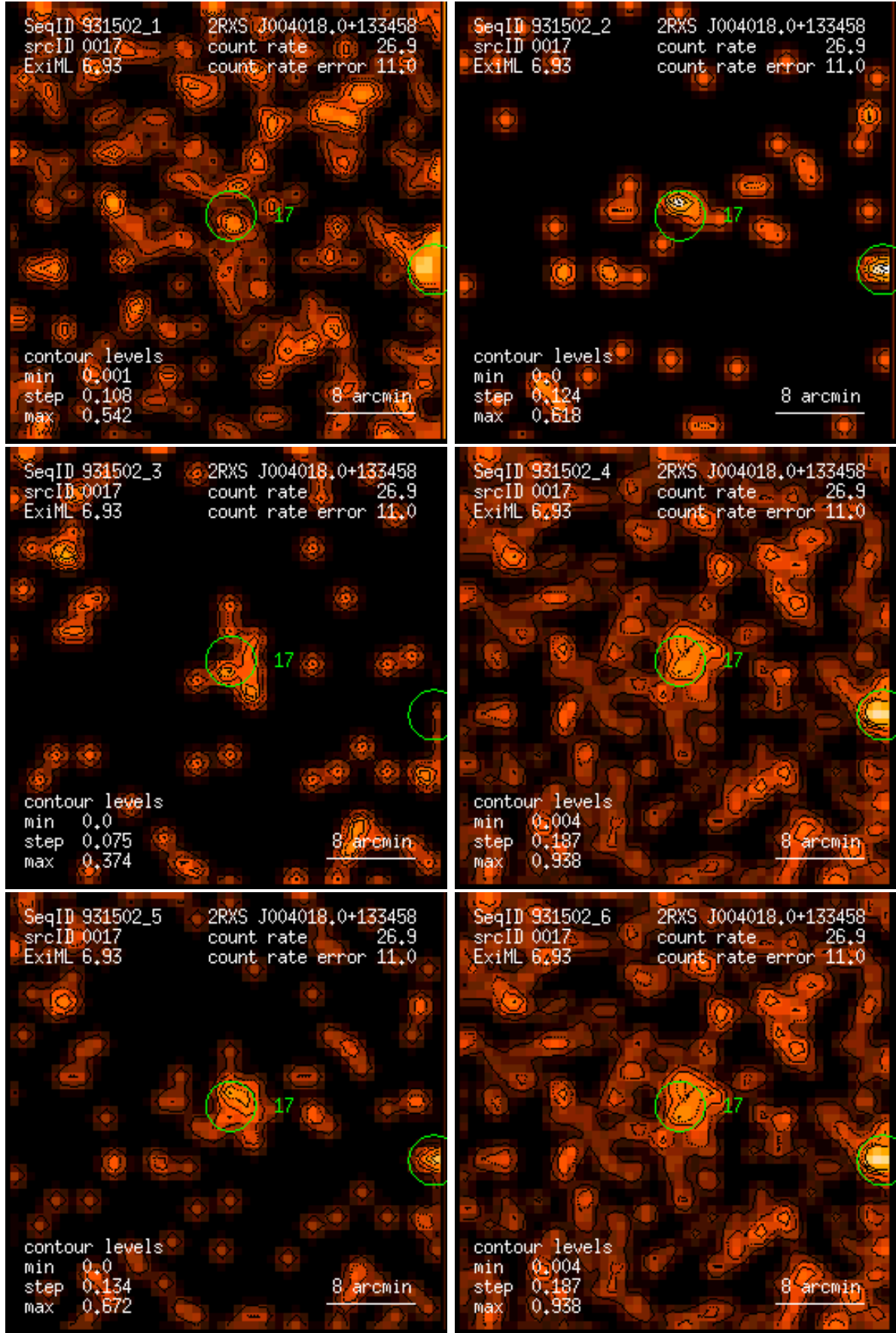
Figure 17: RASS 931502: detection 0017: band rate images, Gaussian filter: (1) PSPC channels 11 – 41, (2) 52 – 90, (3) 91 – 201, (4) 11 – 235, (5) 52 – 201, (6) 11 – 201. Broad band rates in counts/ks. Band rate contour levels in counts/ks/arcmin 2 .
