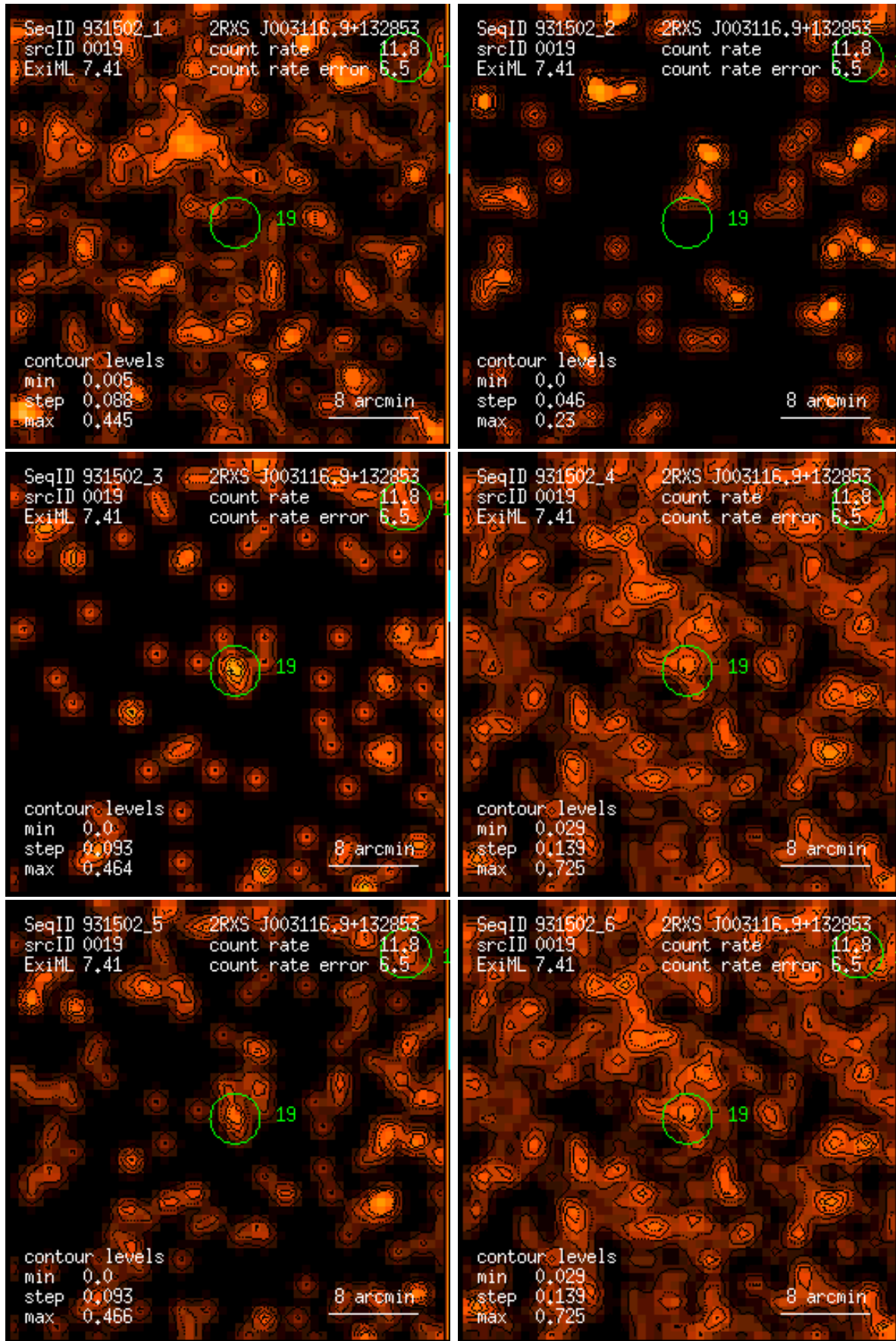
Figure 19: RASS 931502: detection 0019: band rate images, Gaussian filter: (1) PSPC channels 11 – 41, (2) 52 – 90, (3) 91 – 201, (4) 11 – 235, (5) 52 – 201, (6) 11 – 201. Broad band rates in counts/ks. Band rate contour levels in counts/ks/arcmin 2 .
