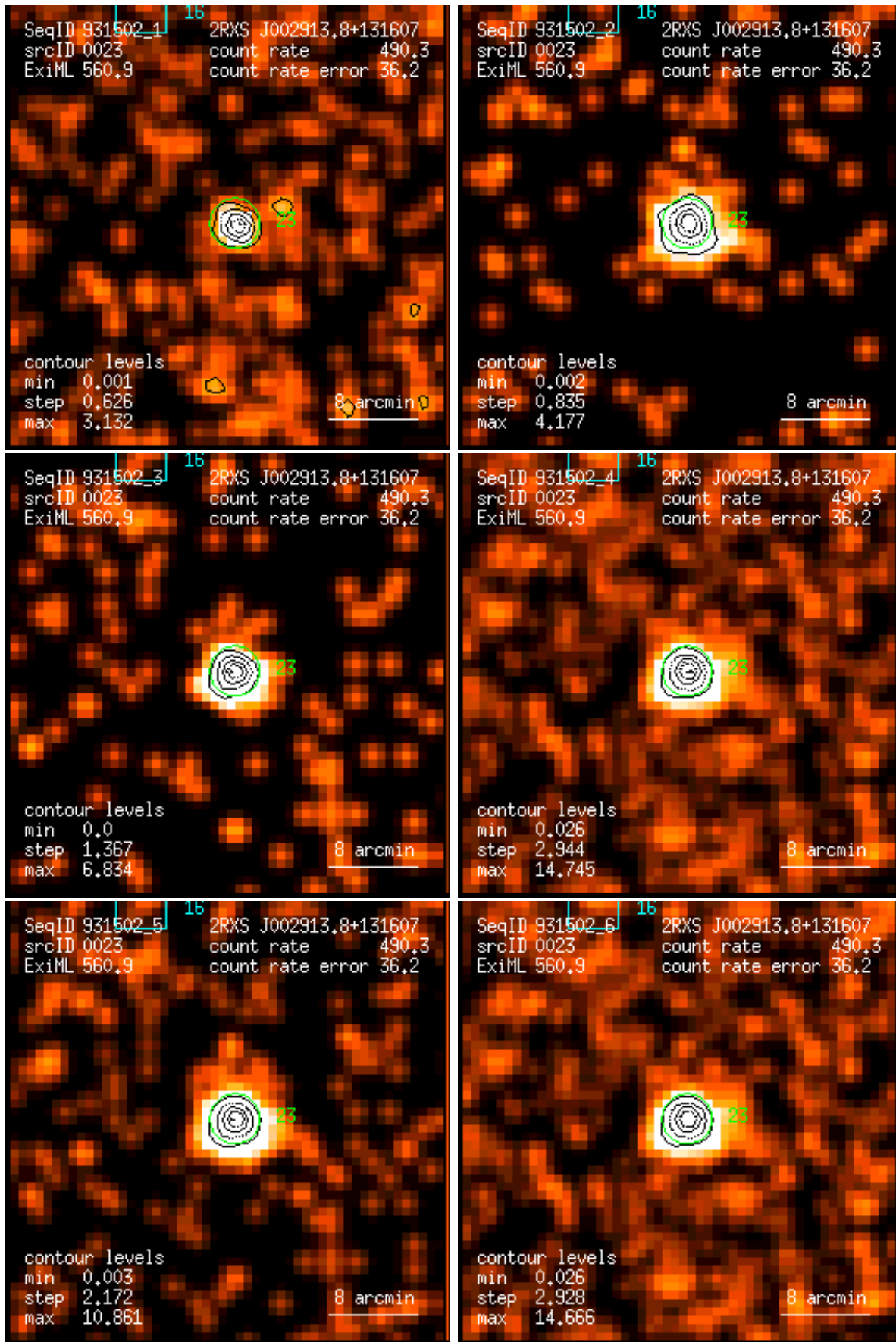
Figure 23: RASS 931502: detection 0023: band rate images, Gaussian filter: (1) PSPC channels 11 – 41, (2) 52 – 90, (3) 91 – 201, (4) 11 – 235, (5) 52 – 201, (6) 11 – 201. Broad band rates in counts/ks. Band rate contour levels in counts/ks/arcmin 2 .
