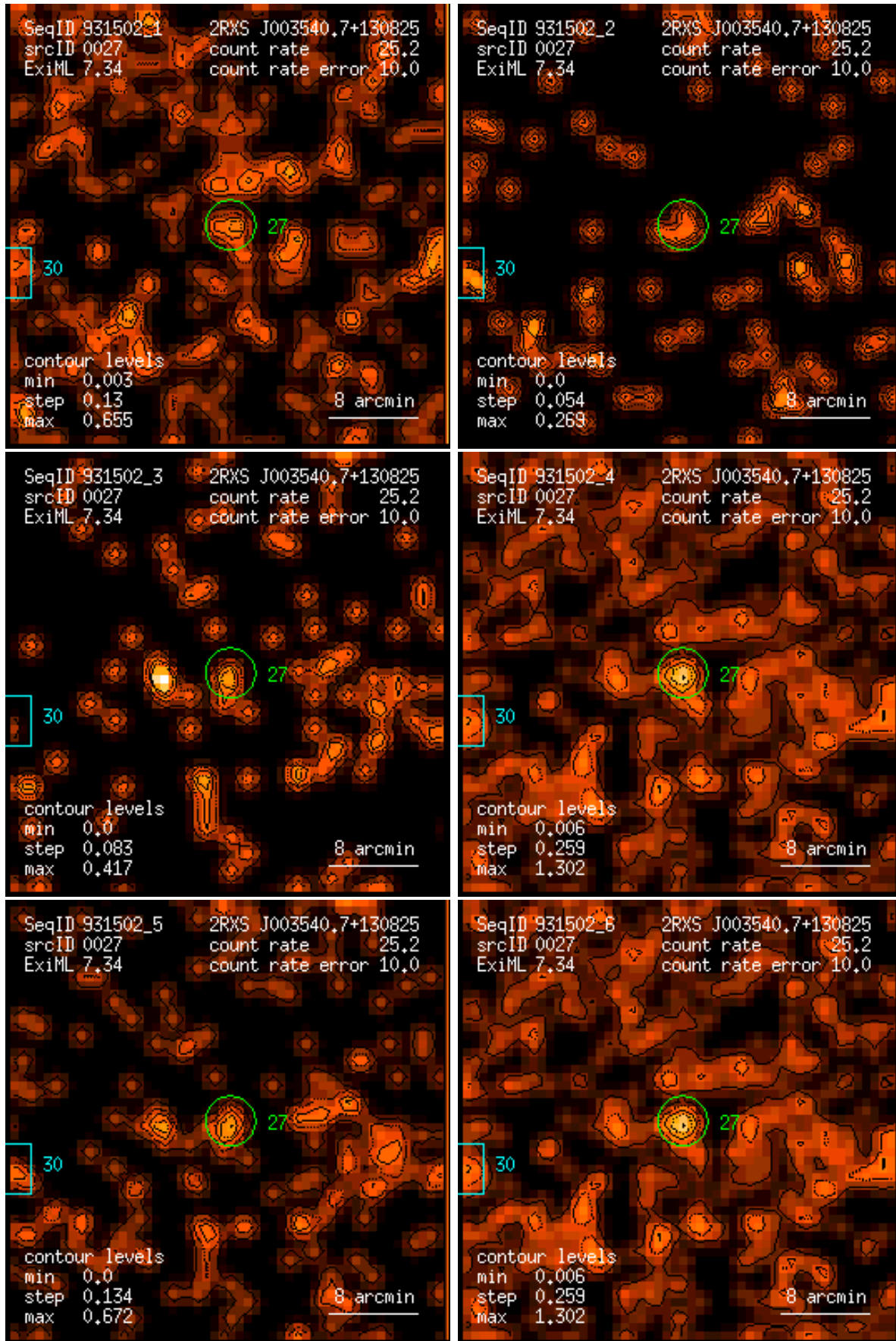
Figure 27: RASS 931502: detection 0027: band rate images, Gaussian filter: (1) PSPC channels 11 – 41, (2) 52 – 90, (3) 91 – 201, (4) 11 – 235, (5) 52 – 201, (6) 11 – 201. Broad band rates in counts/ks. Band rate contour levels in counts/ks/arcmin 2 .
