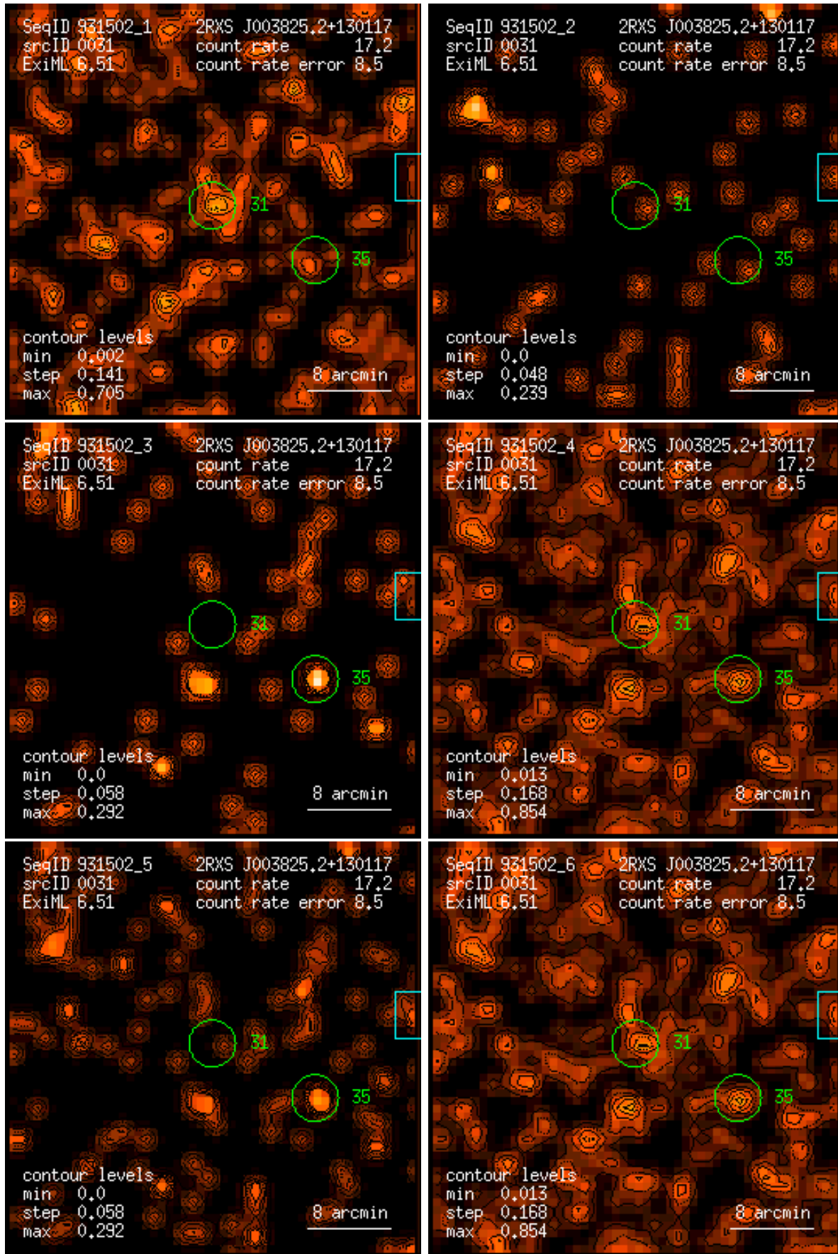
Figure 31: RASS 931502: detection 0031: band rate images, Gaussian filter: (1) PSPC channels 11 – 41, (2) 52 – 90, (3) 91 – 201, (4) 11 – 235, (5) 52 – 201, (6) 11 – 201. Broad band rates in counts/ks. Band rate contour levels in counts/ks/arcmin 2 .
