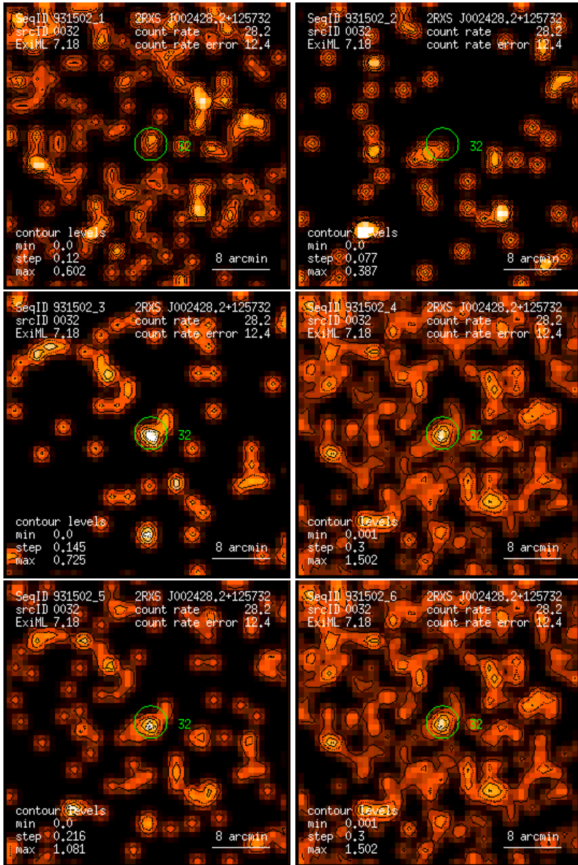
Figure 32: RASS 931502: detection 0032: band rate images, Gaussian filter: (1) PSPC channels 11 – 41, (2) 52 – 90, (3) 91 – 201, (4) 11 – 235, (5) 52 – 201, (6) 11 – 201. Broad band rates in counts/ks. Band rate contour levels in counts/ks/arcmin 2 .
