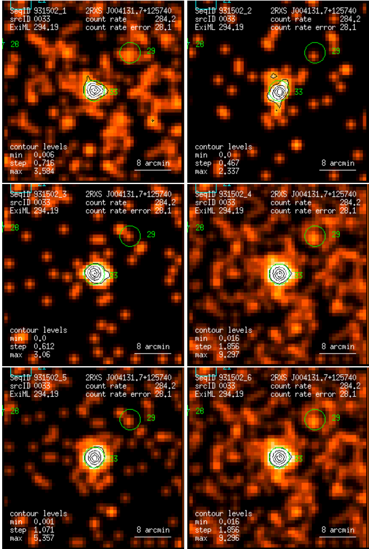
Figure 33: RASS 931502: detection 0033: band rate images, Gaussian filter: (1) PSPC channels 11 – 41, (2) 52 – 90, (3) 91 – 201, (4) 11 – 235, (5) 52 – 201, (6) 11 – 201. Broad band rates in counts/ks. Band rate contour levels in counts/ks/arcmin 2 .
