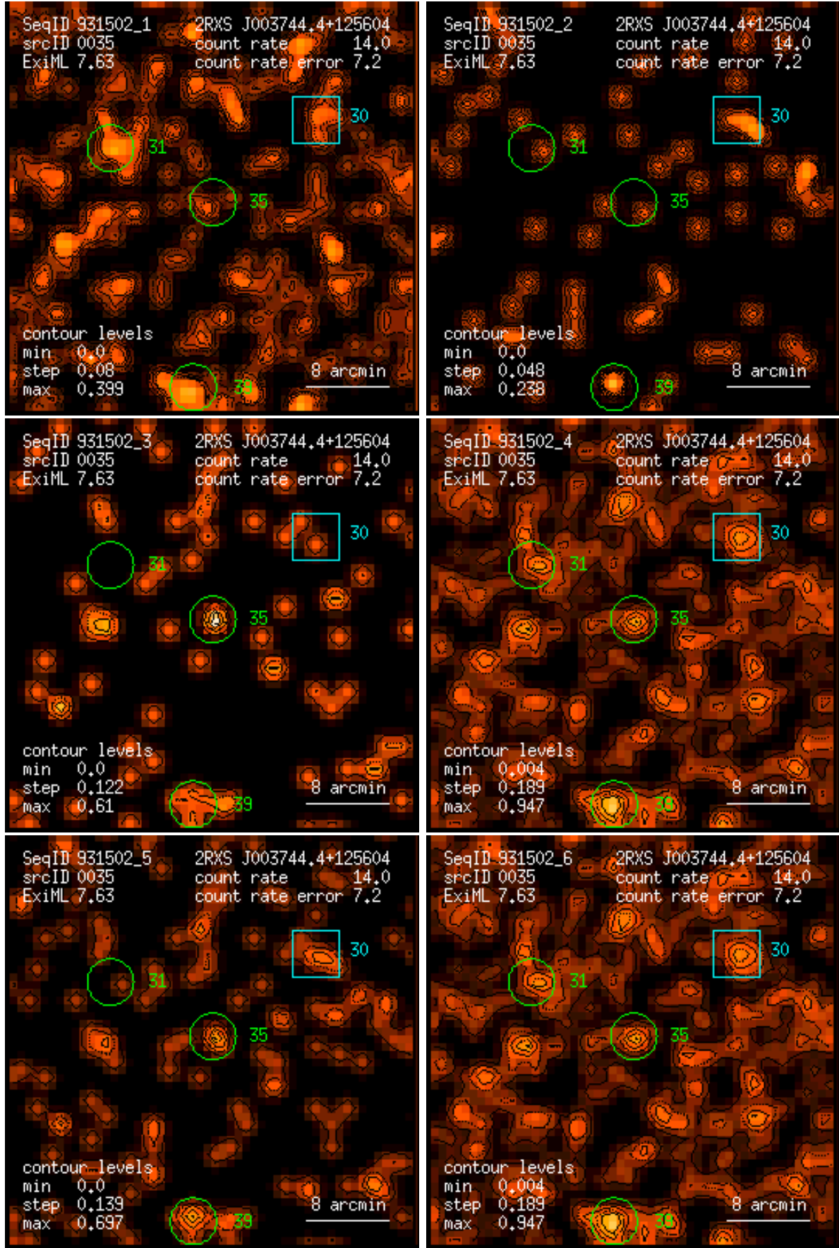
Figure 35: RASS 931502: detection 0035: band rate images, Gaussian filter: (1) PSPC channels 11 – 41, (2) 52 – 90, (3) 91 – 201, (4) 11 – 235, (5) 52 – 201, (6) 11 – 201. Broad band rates in counts/ks. Band rate contour levels in counts/ks/arcmin 2 .
